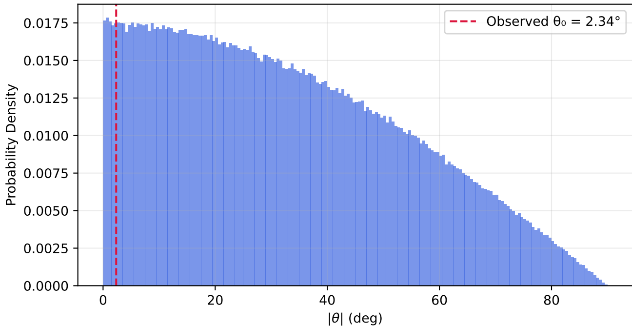
Isotropic Plane-Angle Distribution — ECLIPTIC
