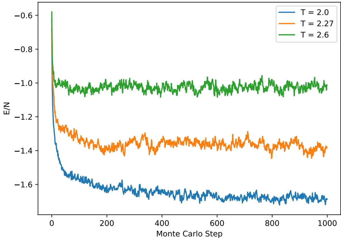
Energy evolution (first 1000 MCS)
