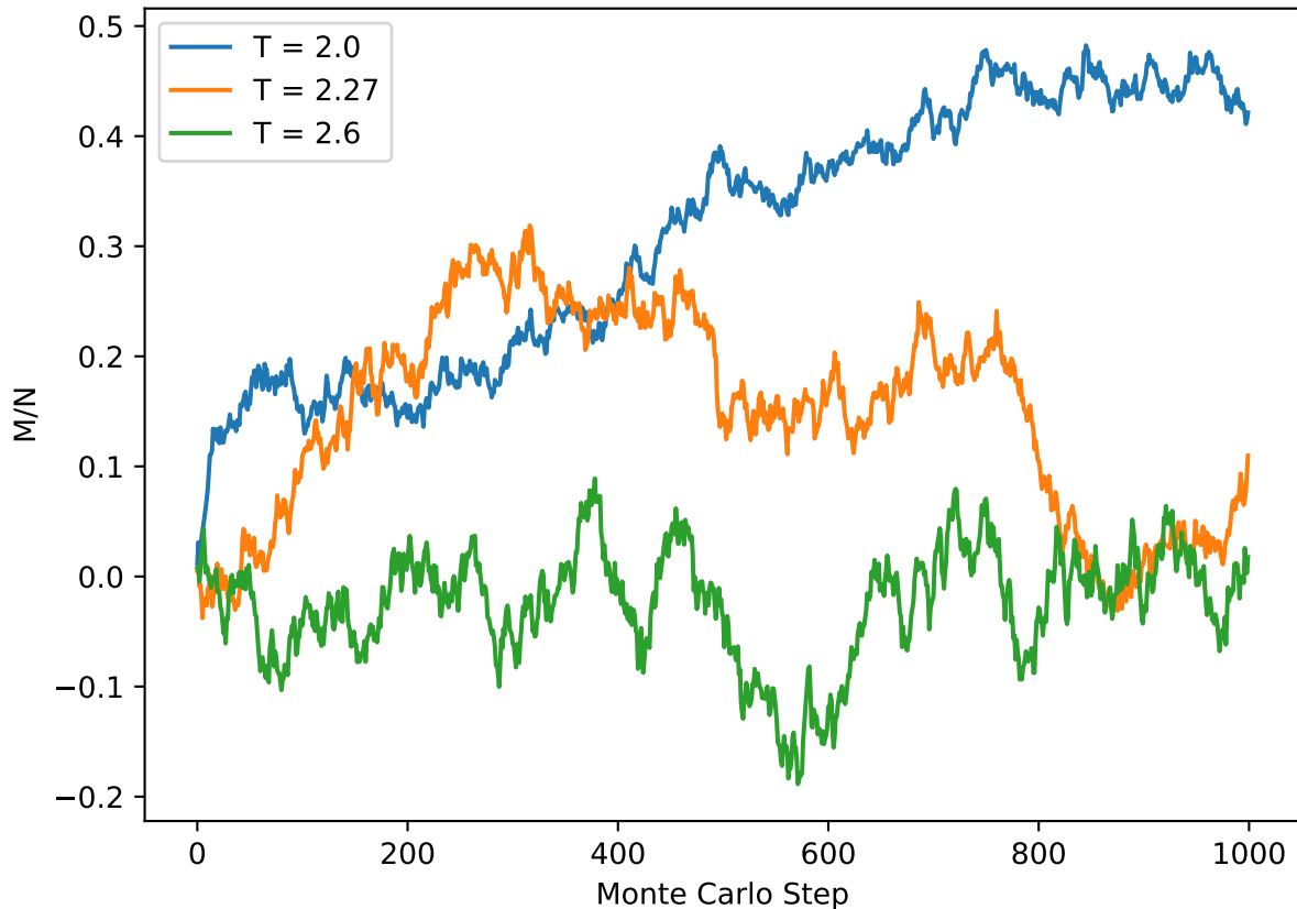
Magnetization evolution (first 1000 MCS)
