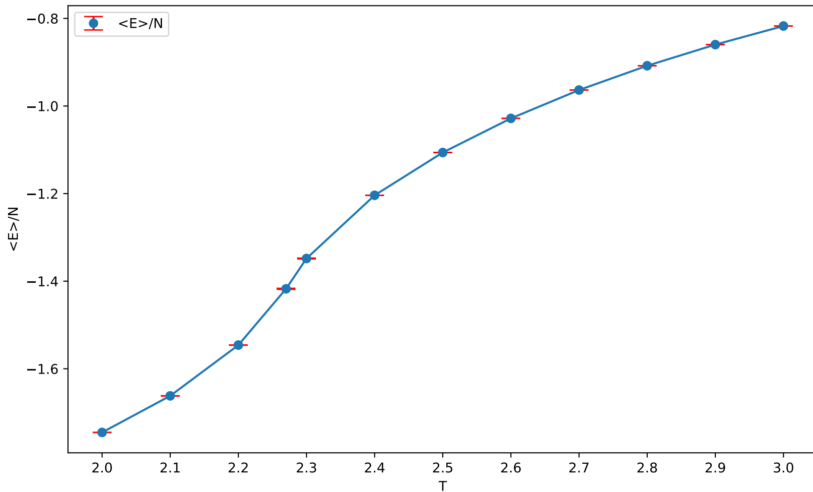
\langle E \rangle / N vs T
