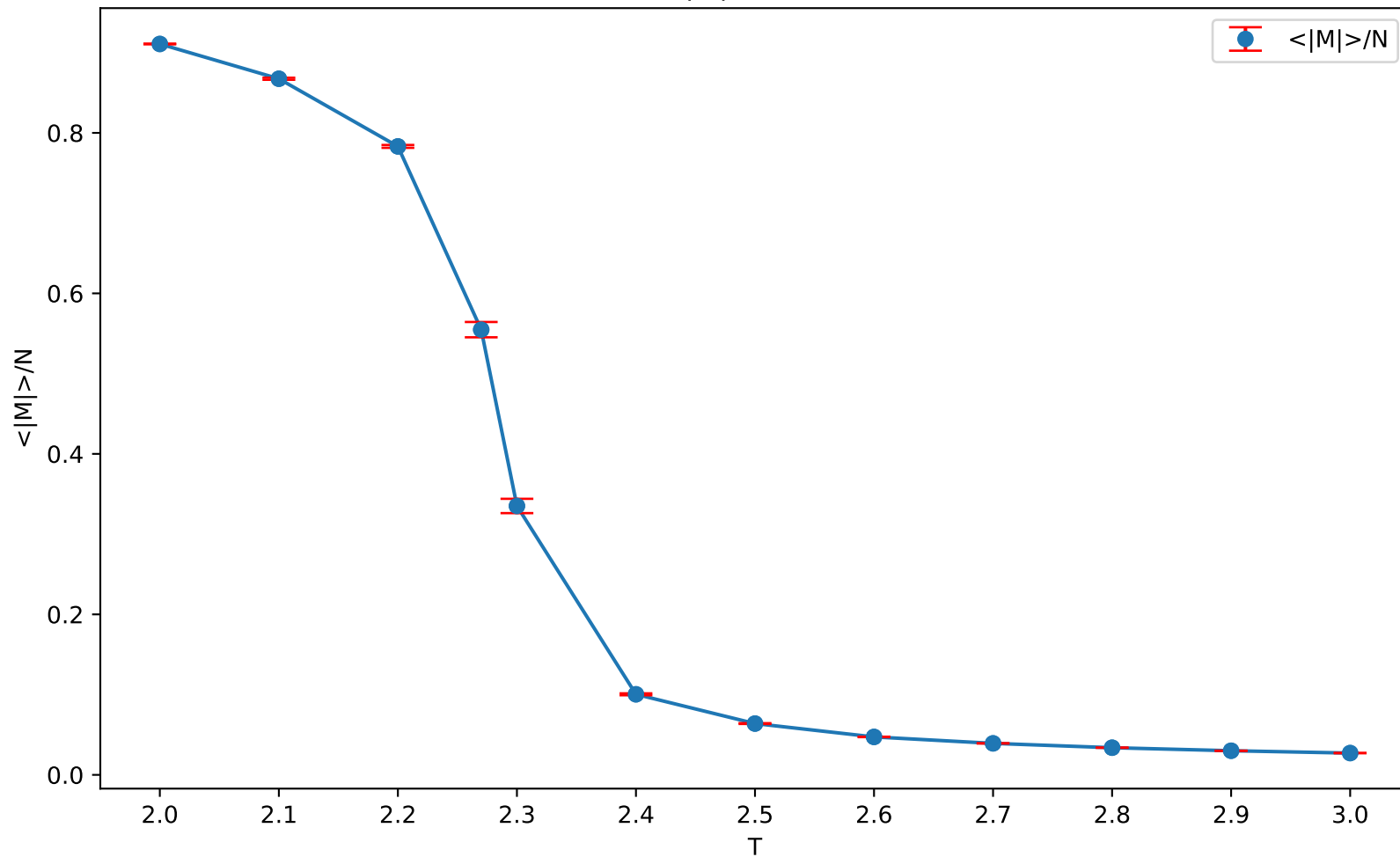
\langle |M| \rangle / N vs T
