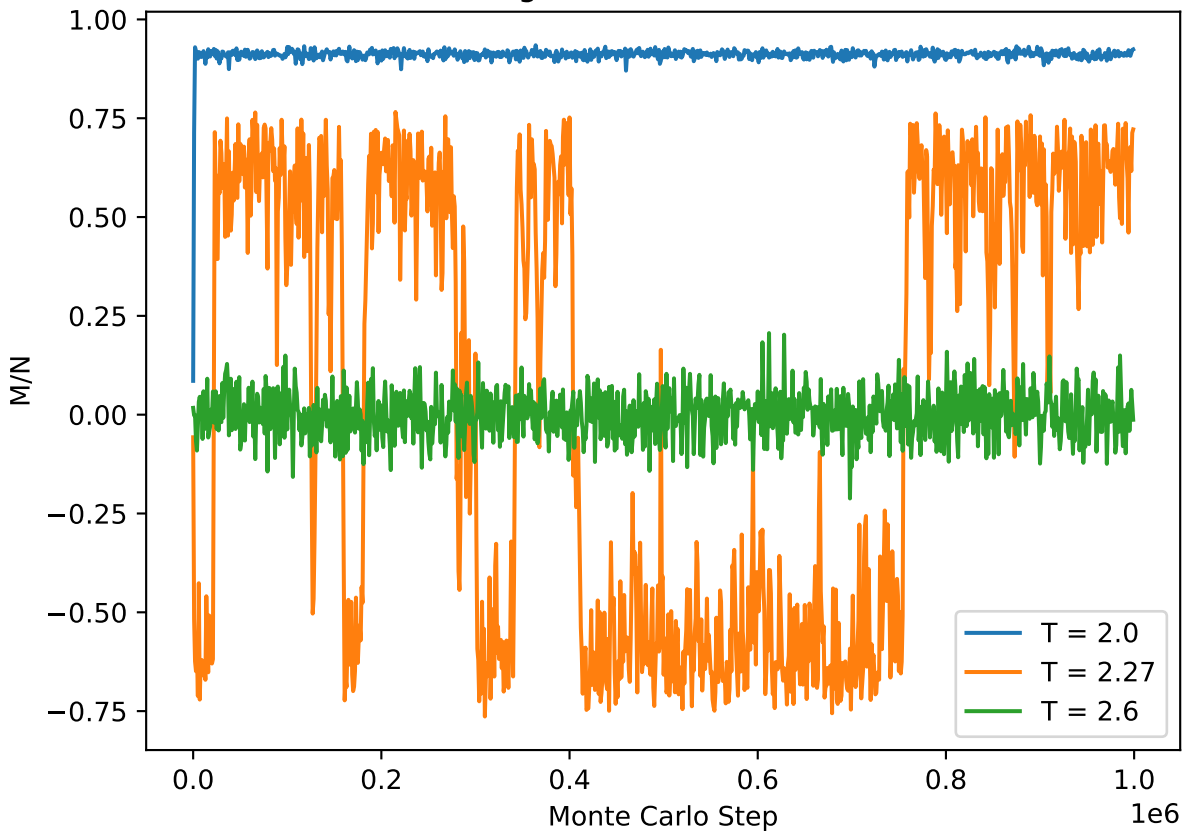
Magnetization evolution
