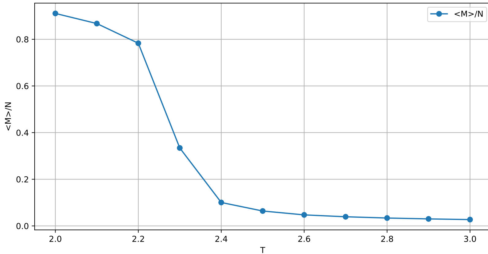
\langle M \rangle / N vs T
