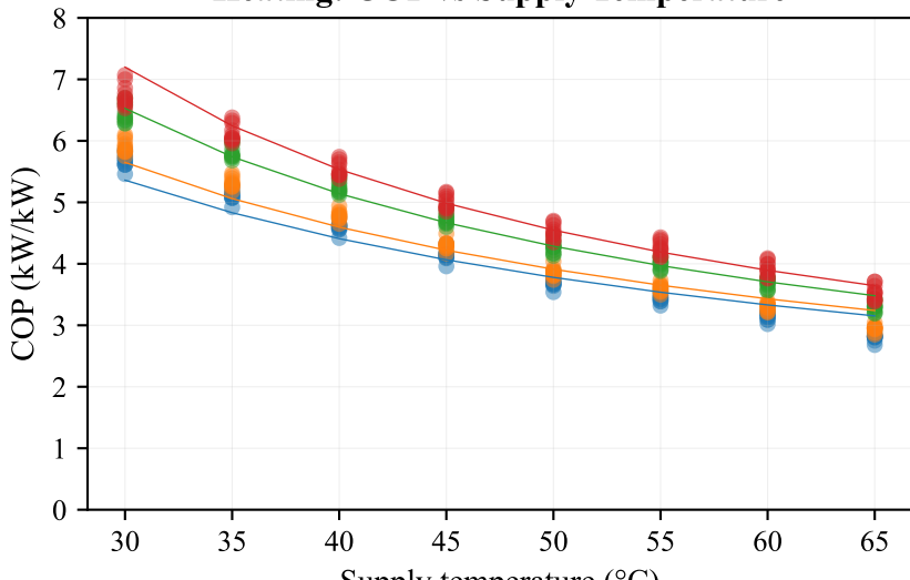
Heating: COP vs Supply Temperature
