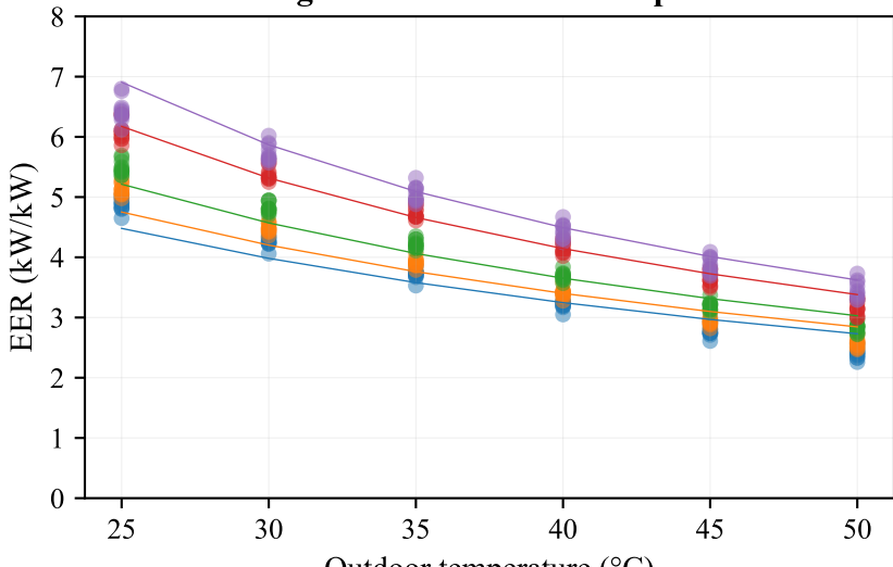
Cooling: EER vs Outdoor Temperature
