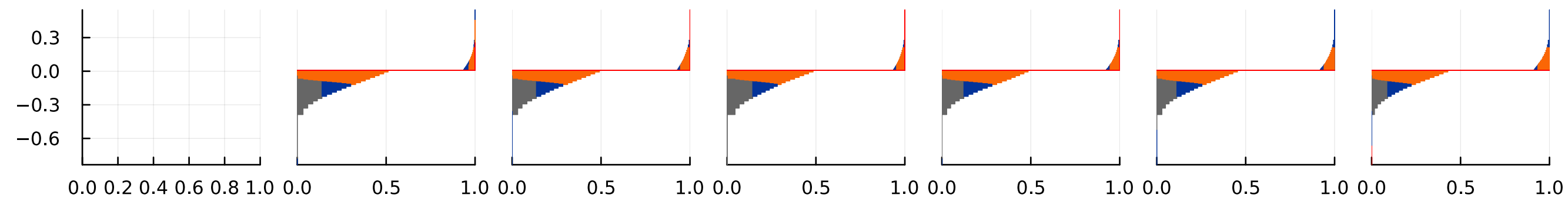
SSP 5.85
