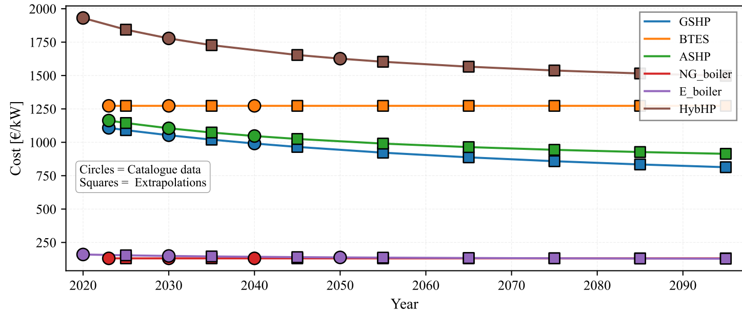
Technology Investment Costs: Historical Data and Projections
