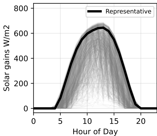
TP 12 ( p=0.07 , avg=268.66) RMSE: 104.281
