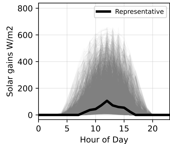
TP 11 ( p=0.08 , avg=69.02) RMSE: 119.298
