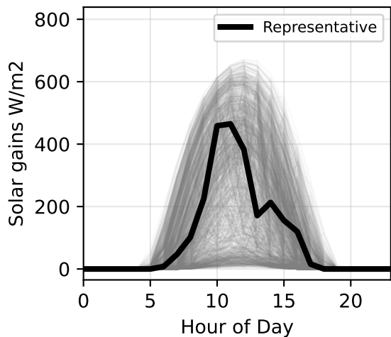
TP 8 ( p=0.03 , avg=261.80) RMSE: 133.021
