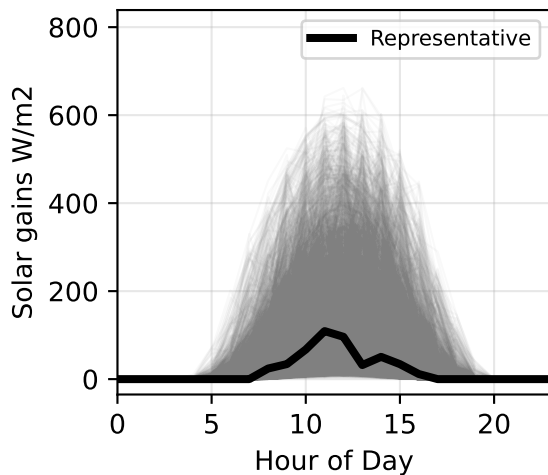
TP 9 ( p=0.07 , avg=36.06) RMSE: 99.672
