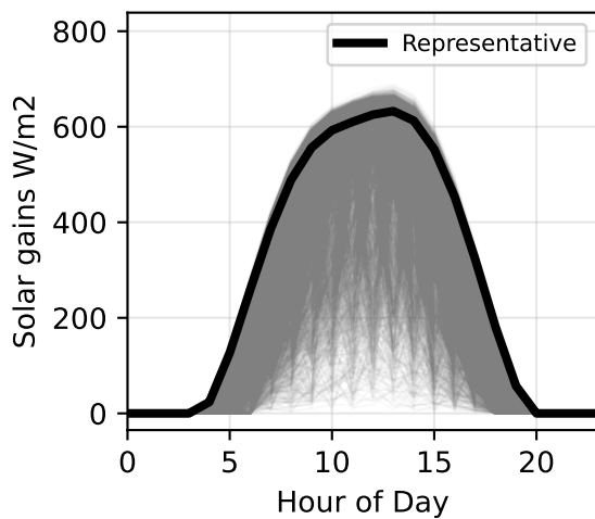
TP 13 ( p=0.08 , avg=270.10) RMSE: 114.718
