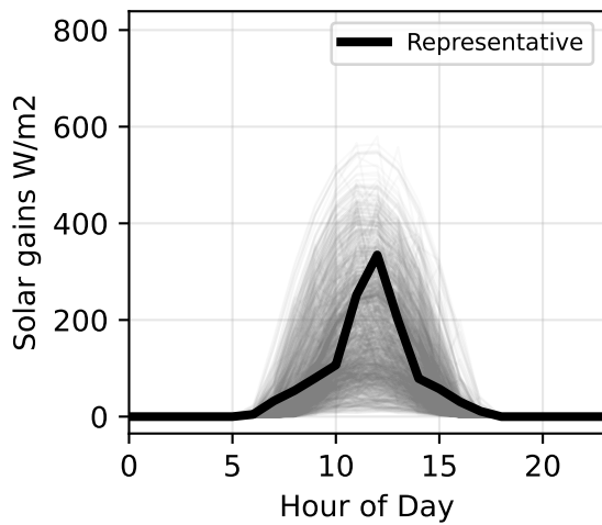
TP 5 ( p=0.15 , avg=19.13) RMSE: 52.225
