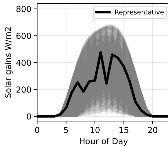
TP 14 ( p=0.03 , avg=259.55) RMSE: 69.755
