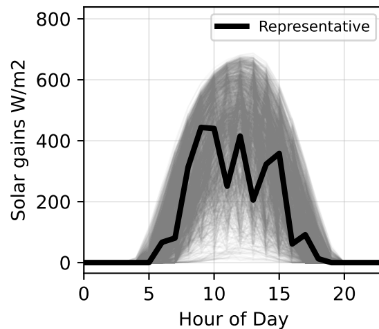
TP 10 ( p=0.08 , avg=151.38) RMSE: 123.142
