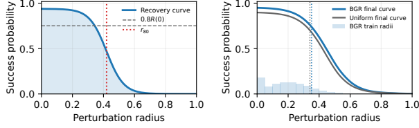
Figure 1: Geometric intuition for BGR and empirical grid-margin trace. Left: a recovery curve maps perturbation radius to success probability, and the critical radius is the success–failure crossing relative to clean success. Right: a deterministic seed-0 grid-margin replay trace overlays final BGR/uniform recovery curves with the BGR training-radius histogram, showing how boundary-centered replay concentrates updates near the trainable transition while retaining coverage.
