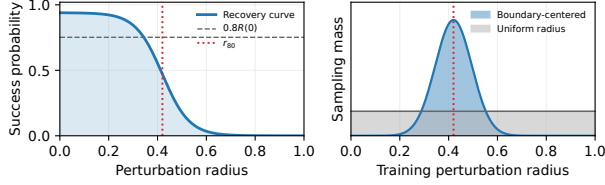
Figure 1: Geometric intuition for BGR. A recovery curve maps perturbation radius to success probability; the critical radius is the success–failure crossing relative to clean success. BGR concentrates radius samples near this crossing while retaining clean, easier, harder, broad, and uniform components for coverage.
