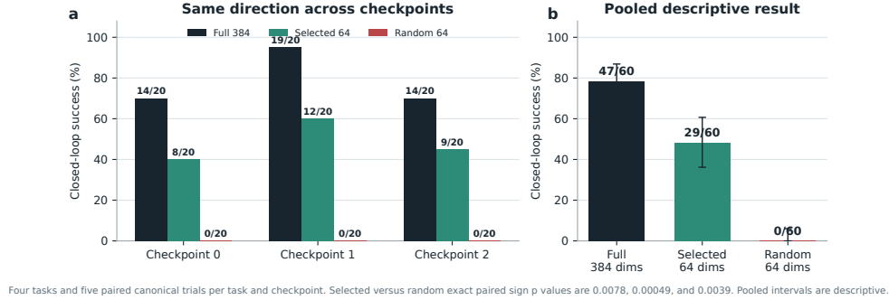
Figure 5: The selected visual subspace has a replicated causal effect, but it is not near-lossless. Each checkpoint uses four tasks and five paired canonical trials per task. Selected subspaces beat random controls in all three checkpoints. The pooled interval is descriptive because trials within a checkpoint share learned weights.
