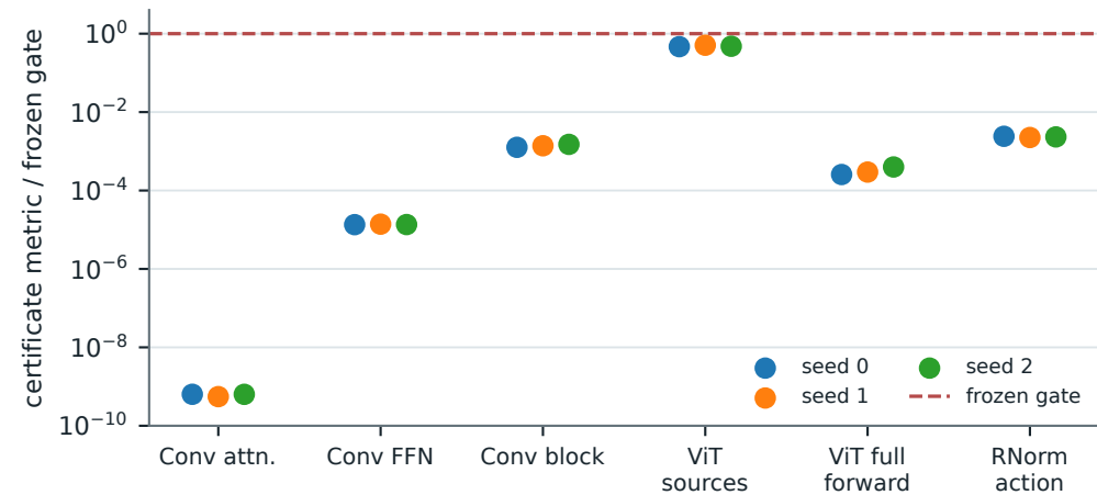
a Independent reconstruction certificates
