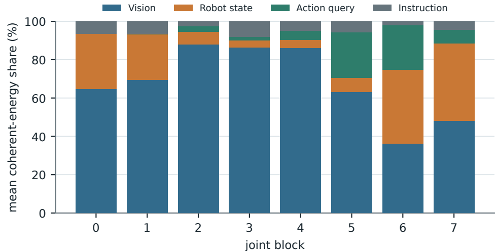
b ViT attention source partition by depth
