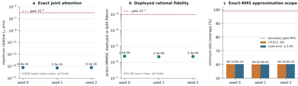
Figure 4: Frozen structural certificates on three independent convolutional checkpoints. Panels (a) and (b) pass their primary gates with large margins. Panel (a) reconstructs all 4,608 audited joint-attention head-input cases. Panel (b) compares deployed float32 normalization with an otherwise identical pass that recomputes only RationalNorm scales in float64. Panel (c) reports the separately frozen exact-RMS approximation coverage, which does not pass its 99% secondary gate.
