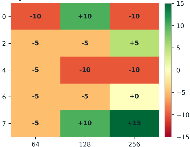
Keep selected minus matched random
