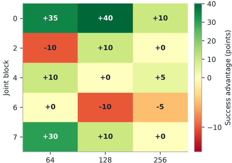
Matched random removal minus selected removal
