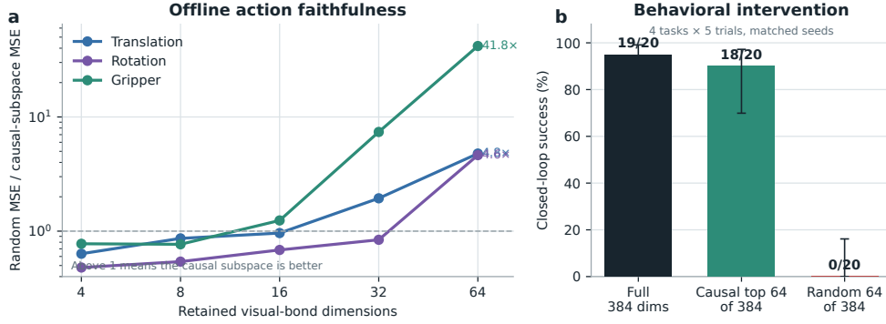
Figure 5: Causally selected visual directions preserve policy behavior. The left panel reports random MSE divided by selected-subspace MSE. The right panel intervenes on the real policy over four tasks and five paired trials per task.
