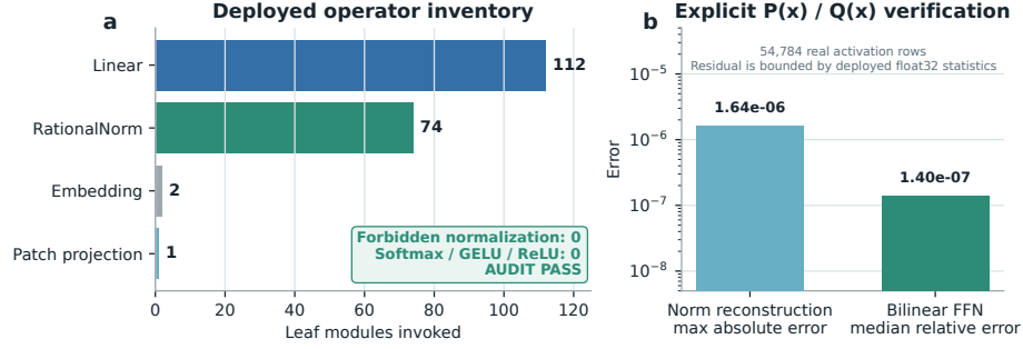
Figure 1: Mechanical audit of the seed-0 20.1M ViT rational checkpoint. The runtime path invokes 112 linear maps, 74 rational normalizers, two embeddings, and one linear patch projection. No softmax, standard activation, or ordinary normalization is present. Reconstruction errors are measured over 54,784 real activation rows.
