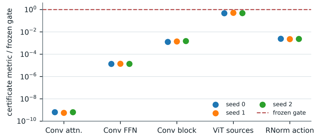
a Independent reconstruction certificates
