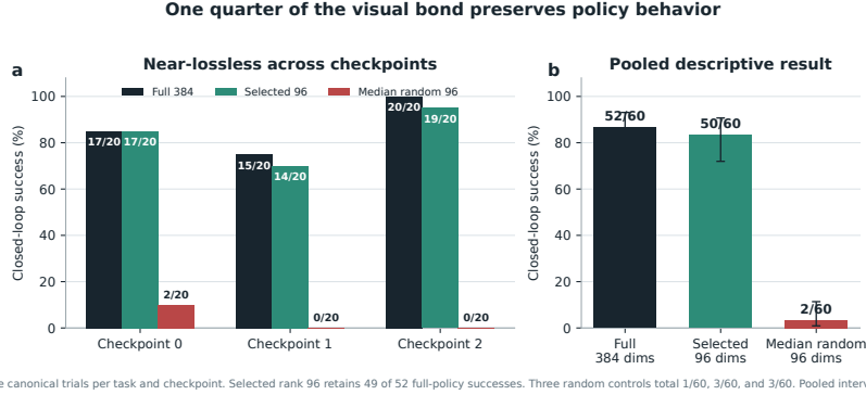
Figure 3: One quarter of the visual bond preserves policy behavior. Each checkpoint uses four tasks and five paired canonical trials per task. Rank 96 retains 49 of 52 full-policy successes. Three equal-rank random controls reach 1/60, 3/60, and 3/60. The pooled interval is descriptive because trials within a checkpoint share learned weights.
