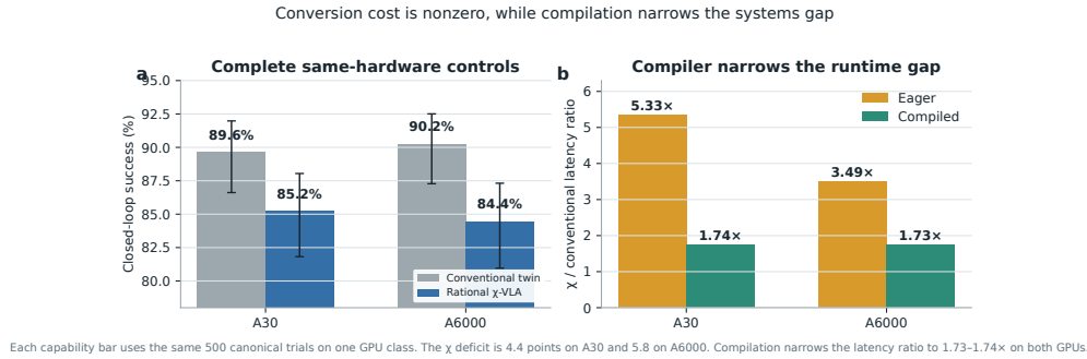
Figure 6: Conversion cost is modest but nonzero, and compilation narrows the systems gap. Complete same-hardware evaluations give 89.6% versus 85.2% on A30 and 90.2% versus 84.4% on A6000, conventional then rational. Parameters differ by 0.006%. Compilation narrows the batch-one latency ratio to 1.73–1.74x on both GPUs.
