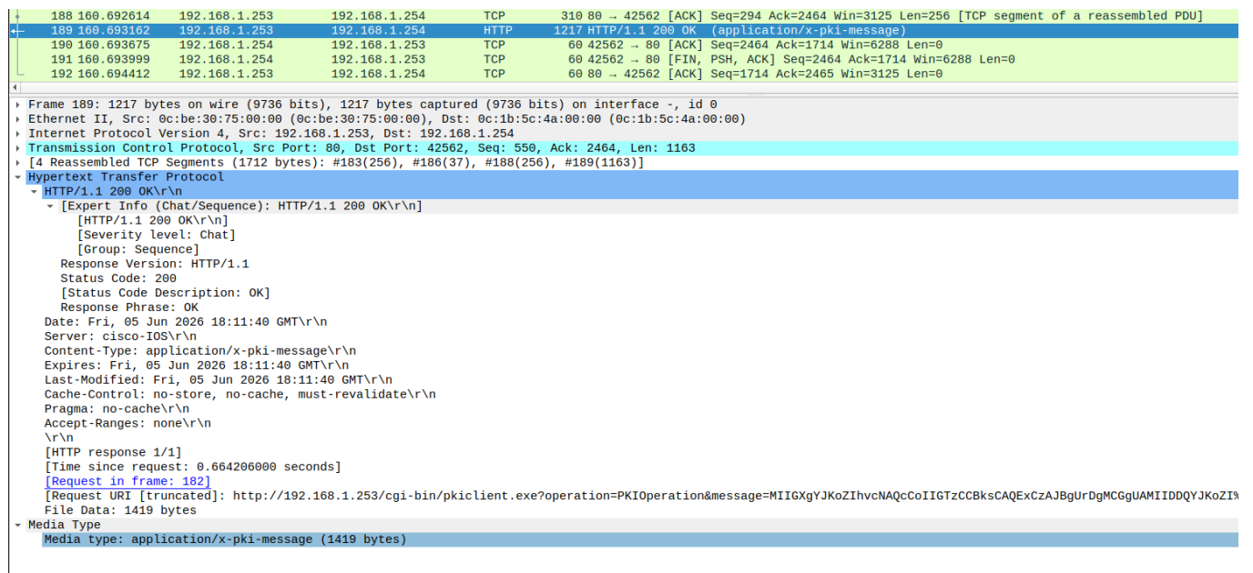
Figure 42: CA response delivering the signed certificate: 200 OK (application/x-pki-message).
