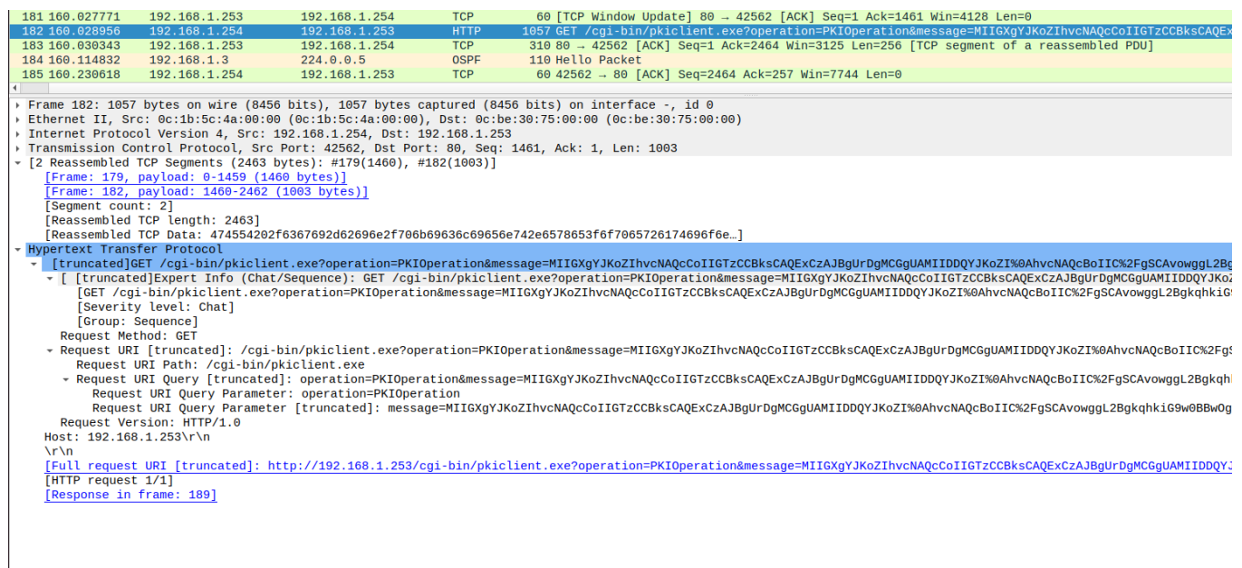
Figure 41: HTTP GET from R1 carrying the base64-encoded CSR (operation=PKIOperation).
