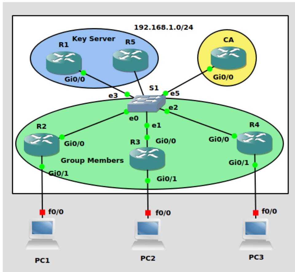
Figure 36: Updated topology with the CA server added at 192.168.1.253.
