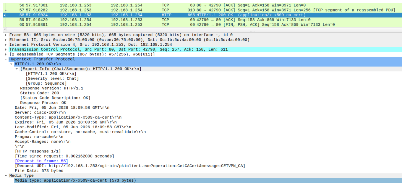
Figure 40: CA response delivering its certificate: 200 OK (application/x-x509-ca-cert).
