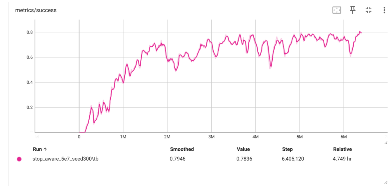
Fig. 7 TensorBoard success curve — no saturation at 5e7 (grad_norm 15.97→7.47)
