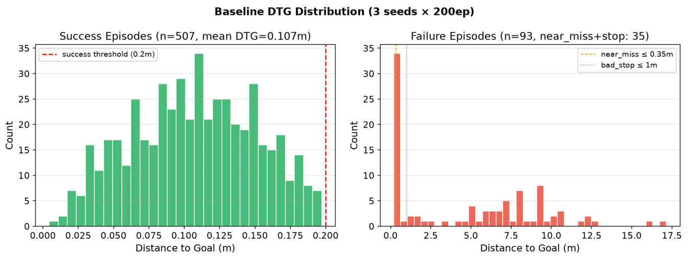
Fig. 2 Baseline DTG distribution — near-miss failures sit just 0.01 m outside the 0.2 m success radius
