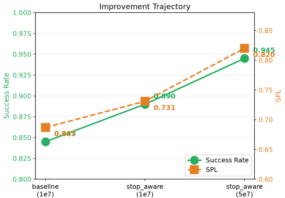
Fig. 6 Improvement trajectory — steps are the highest-leverage change; curves keep improving with no saturation
