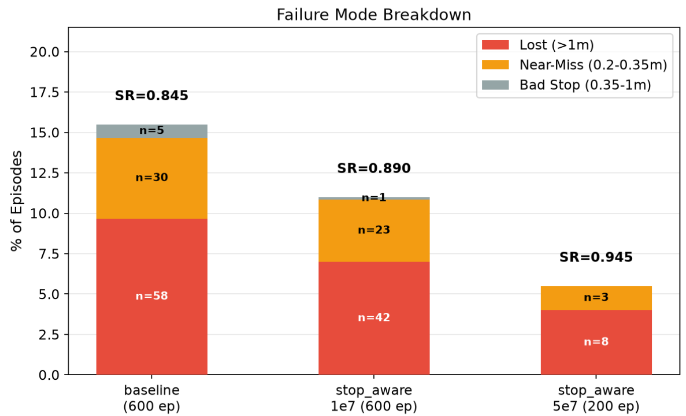
Fig. 4 Failure modes — stop-aware fixes stop-related failures; 5e7 further cuts lost episodes
