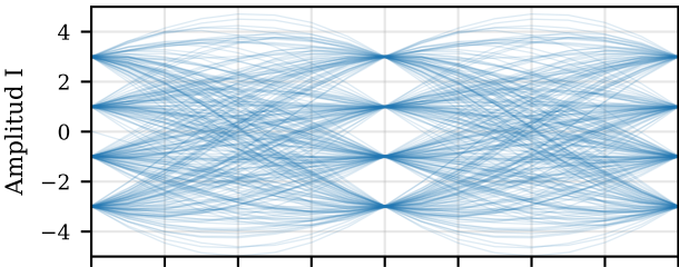
(b) AWGN, E_b/N_0 = 14 dB
