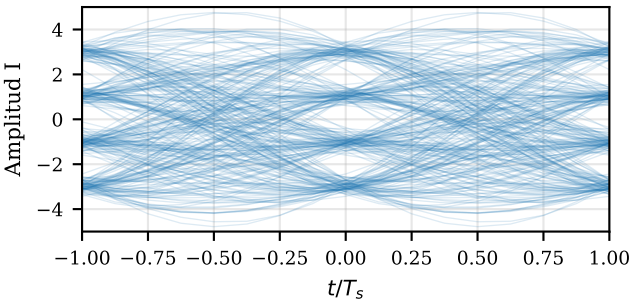
(b) AWGN, E_b/N_0 = 14 dB
