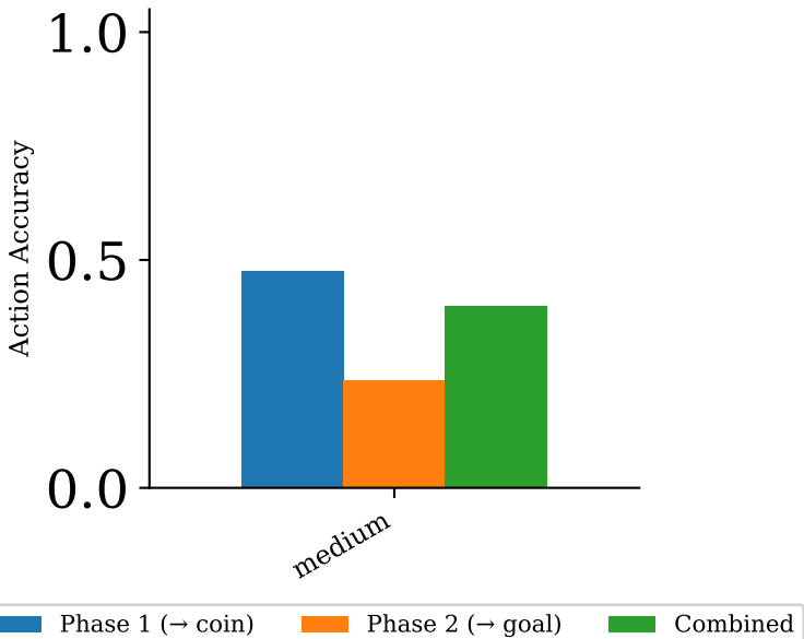
Phase Action Accuracy — medium
