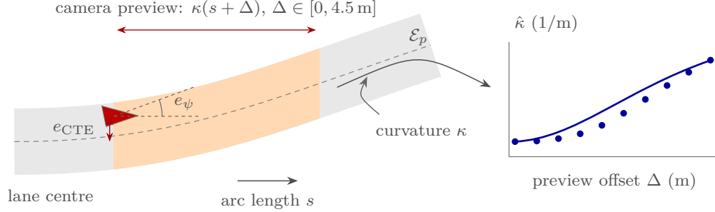
Figure 3: Encoding the road environment. The road-context state z^r = (e_{\text{CTE}}, e_{\psi}, \kappa) is defined geometrically with respect to the lane centre: the cross-track error is the signed lateral offset, the heading error is the angle between the vehicle heading and the road tangent, and \kappa is the local curvature. For a forward-facing camera the road is visible only over a short preview (shaded), so the physical encoder \mathcal{E}_p aggregates a temporal window of images into a curvature profile \hat{\kappa}(s + \Delta) sampled at ten offsets over the first 4.5 m ahead. On the real DonkeyCar this encoding is supervised by privileged track localization at training time and recovered from the front camera alone at test time.
