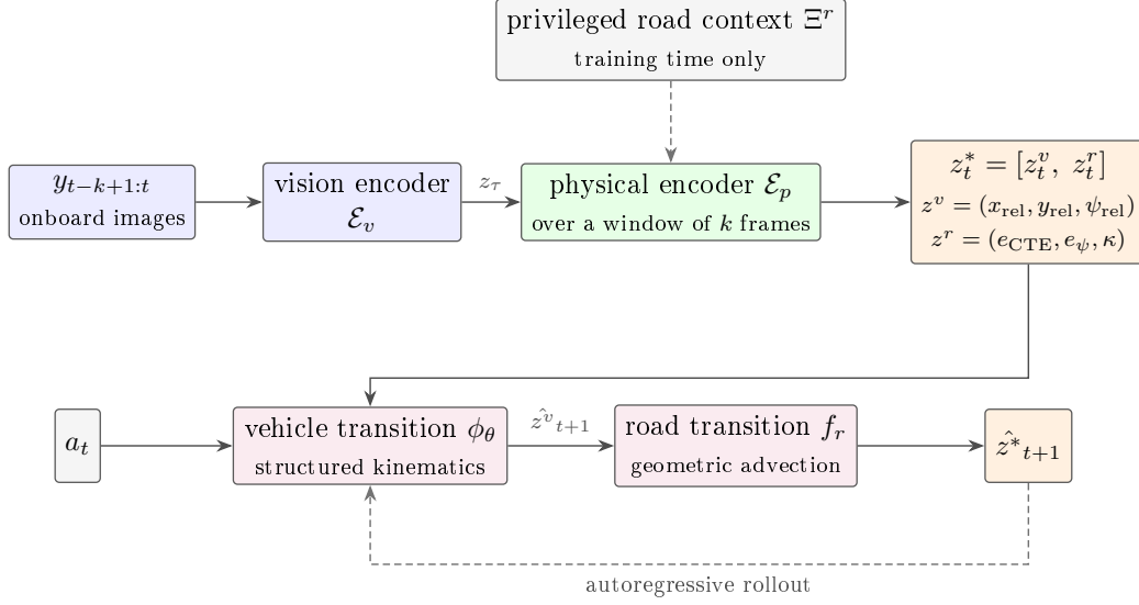
Figure 2: Overview of the PIWM architecture for partially observable driving. A vision encoder maps each observation to a visual latent; a physical encoder aggregates a temporal window of those latents into the factorized interpretable state z^* = [z^v, z^r] , where z^v is the vehicle-relative state and z^r the road context. A split-dynamics model then rolls the state forward, advancing z^v with a structured kinematic model and z^r with a geometry-driven transition that advects the road past the vehicle. The encoder (Section 5.2) infers the external road environment from images, supervised at training time by a privileged signal that is withheld at test time; the predictor (Section 5.3) forecasts how that environment evolves.
