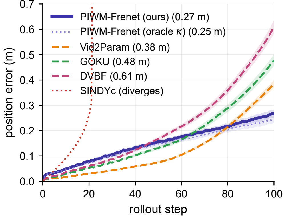
Figure 5: Position error against rollout step on the physical DonkeyCar (mean \pm standard error over the 201 held-out validation windows, all rollouts initialized from the ground-truth state). The baselines lead over short horizons and then enter superlinear growth; the proposed model stays close to linear because the road it rolls out over was observed rather than extrapolated. SindyC leaves the plot range before step 25. The privileged oracle curve (dotted) is our own model with \kappa read from the track map and sits only \sim 2 cm below the perceived model at step 100.
