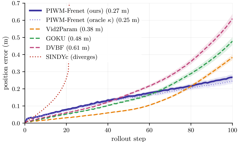
Figure 5: Position error against rollout step on the physical DonkeyCar (mean \pm standard error over the 201 held-out validation windows, all rollouts initialized from the ground-truth state). The baselines lead over short horizons and then enter superlinear growth; the proposed model stays close to linear because the road it rolls out over was observed rather than extrapolated. SINDYc leaves the plot range before step 25. The privileged oracle curve (dotted) is our own model with \kappa read from the track map and sits only \sim 2 cm below the perceived model at step 100.
