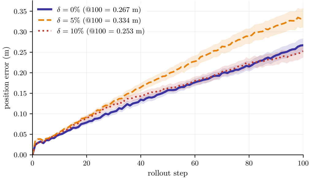
Figure 6: Robustness to corrupted road-context supervision. Position error against rollout step on the physical DonkeyCar when the labels used to train the road-context encoder carry biased uniform noise of relative width \delta . All three curves stay below the 0.383 m reached at step 100 by the strongest baseline trained on clean labels.
