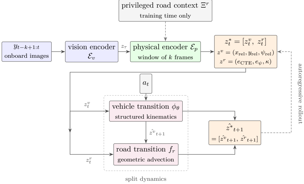
Figure 2: Overview of the PIWM architecture for partially observable driving. A vision encoder maps each observation to a visual latent; a physical encoder aggregates a temporal window of those latents into the factorized interpretable state z^* = [z^v, z^r] , where z^v is the vehicle-relative state and z^r the road context. A split-dynamics model then rolls the state forward: the two components are advanced by separate transitions, z^v by a structured kinematic model and z^r by a geometry-driven one, and the predicted components recombine into \hat{z}_{t+1}^* . Their only coupling is the arrow labeled \hat{z}_{t+1}^v —the road is advected by the vehicle’s own predicted motion, which is also why the action a_t enters the vehicle branch alone. The encoder (Section 5.2) infers the external road environment from images, supervised at training time by a privileged signal that is withheld at test time; the predictor (Section 5.3) forecasts how that environment evolves.
