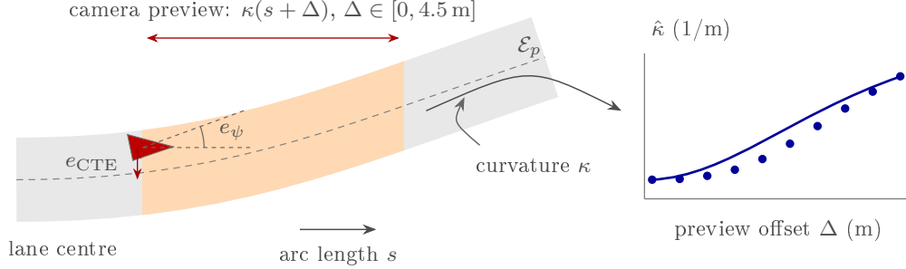
Figure 3: Encoding the road environment. The road-context state z^r = (e_{\text{CTE}}, e_\psi, \kappa) is defined geometrically with respect to the lane centre: the cross-track error is the signed lateral offset, the heading error is the angle between the vehicle heading and the road tangent, and \kappa is the local curvature. For a forward-facing camera the road is visible only over a short preview (shaded), so the physical encoder \mathcal{E}_p aggregates a temporal window of images into a curvature profile \hat{\kappa}(s + \Delta) sampled at ten offsets over the first 4.5m ahead. On the real DonkeyCar this encoding is supervised by privileged track localization at training time and recovered from the front camera alone at test time.
