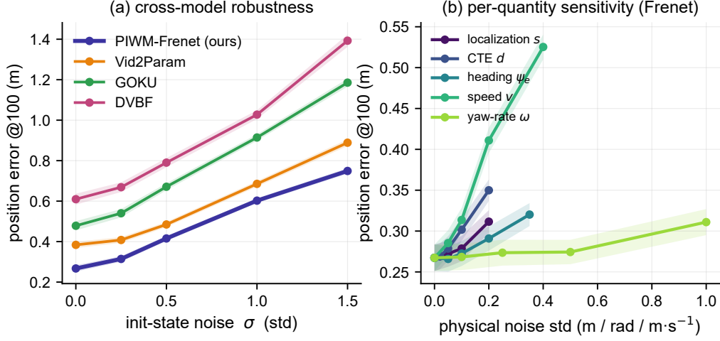
Figure 7: Robustness to a corrupted initial state (test-time perturbation; distinct from the training-label noise of Table 3). (a) 100-step position error against the noise scale \sigma applied to all state variables; the ranking is preserved throughout. (b) Sensitivity of our model to noise on each physical state variable separately. Speed dominates; yaw rate is nearly irrelevant. Shaded bands are standard errors over the 201 validation windows.
