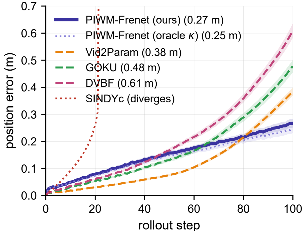
Figure 5: Position error against rollout step on the physical DonkeyCar (mean \pm standard error over the 201 held-out validation windows, all rollouts initialized from the ground-truth state). The baselines lead over short horizons and then enter superlinear growth; the proposed model stays close to linear because the road it rolls out over was observed rather than extrapolated. SindyC leaves the plot range before step 25. The privileged oracle curve (dotted) is our own model with \kappa read from the track map and sits only \sim 2 cm below the perceived model at step 100.
