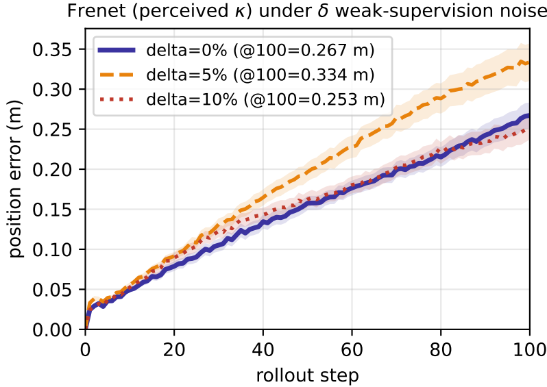
Figure 6: Robustness to corrupted road-context supervision. Position error against rollout step on the physical DonkeyCar when the labels used to train the road-context encoder carry biased uniform noise of relative width \delta . All three curves stay below the 0.383 m reached at step 100 by the strongest baseline trained on clean labels.
