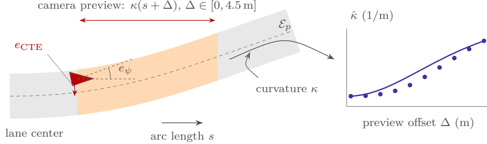
Figure 3: Encoding the road environment. The road-context state z^r = (e_{\text{CTE}}, e_\psi, \kappa) is defined geometrically with respect to the lane center: the cross-track error is the signed lateral offset, the heading error is the angle between the vehicle heading and the road tangent, and \kappa is the local curvature. For a forward-facing camera the road is visible only over a short preview (shaded), so the physical encoder \mathcal{E}_p aggregates a temporal window of images into a curvature profile \hat{\kappa}(s + \Delta) sampled at ten offsets over the first 4.5 m ahead. On the real DonkeyCar this encoding is supervised by privileged track localization at training time and recovered from the front camera alone at test time.
