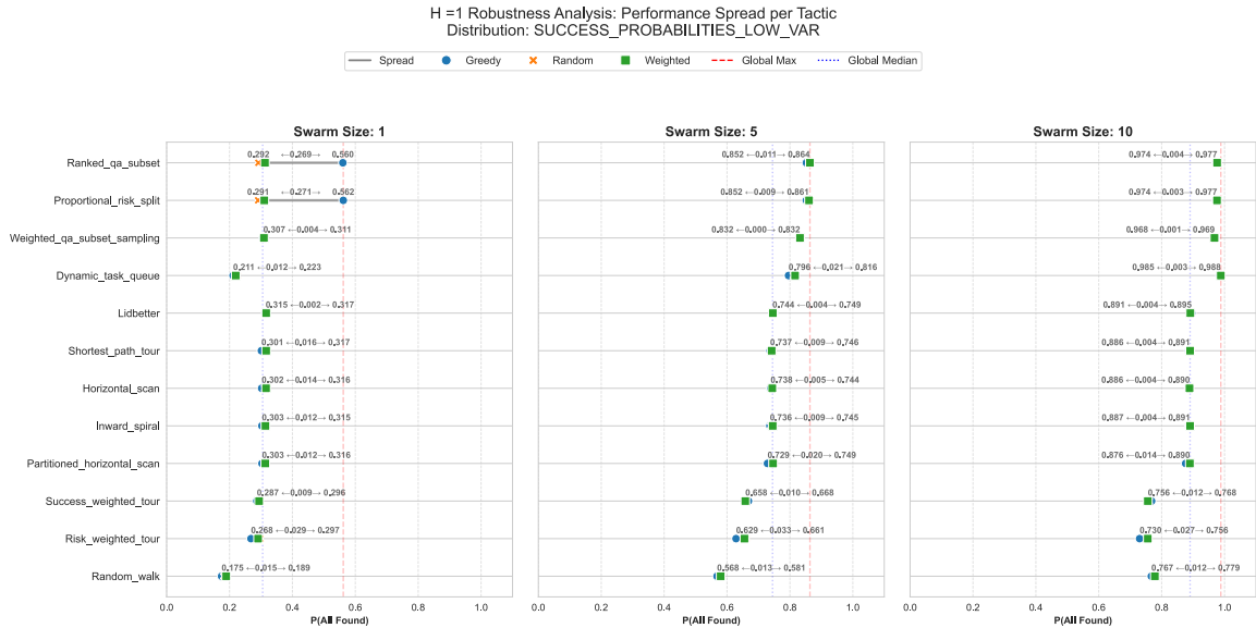
Figure 7: Cleveland dot plot of probability of all hiders found for swarm size 1, 5 and 10, given 1 hiders, 5 possible hiding locations and the different hiding strategies, simulated on a 20 x 20 grid with the low variation probability distribution. The plot shows robustness of strategies, i.e. wider lines could be viewed as less robust.
