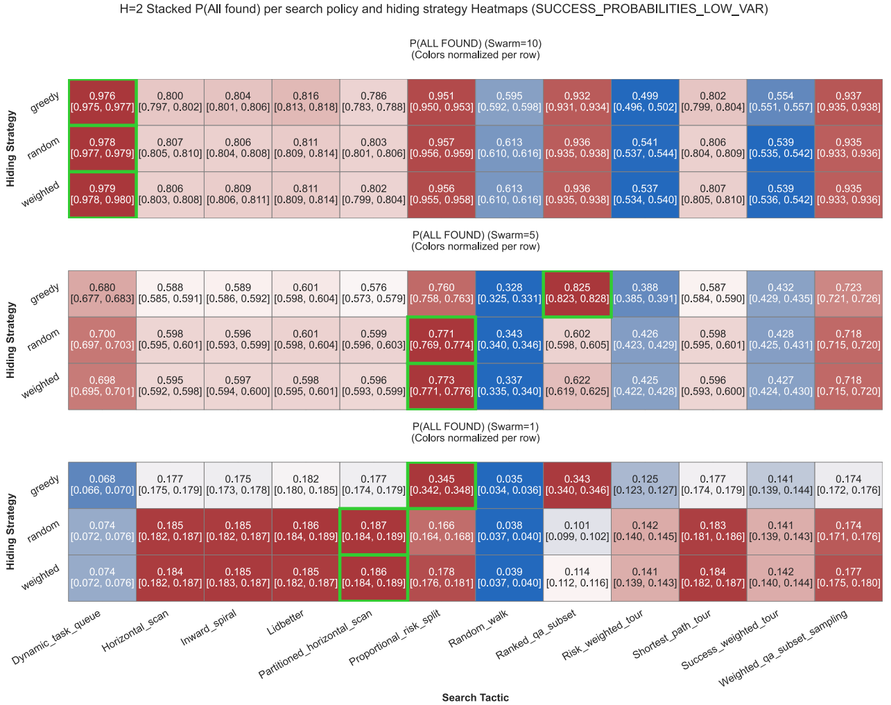
Figure 14: Full stacked heatmap of 2/5 hidrs, all tactics, all hiding strategies, for the low variance probability distribution.
