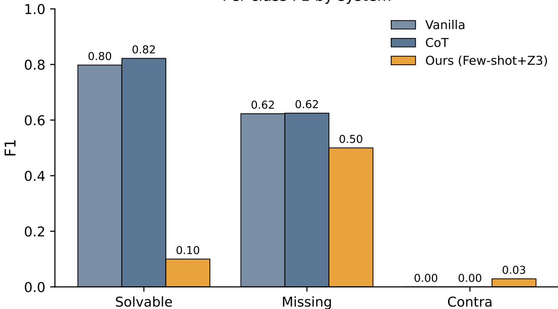
Per-class F1 by system
