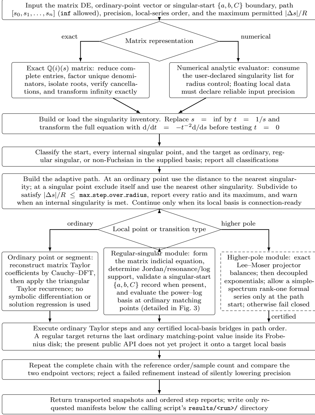
Figure 1: Basic numerical matrix-DE workflow. Input formats and output layout are detailed in Sec. 6.6; exact/numerical representations and ordinary recurrences in Sec. 6.1; singularity inventory and infinity in Sec. 6.1.2; path construction and each |\Delta s|/R report in Sec. 6.1.3; matrix indicial data in Sec. 6.2; the log node in Sec. 6.3; the high-pole module and its fail-closed boundary in Sec. 6.4; and transport/refinement in Sec. 6.6.3.
