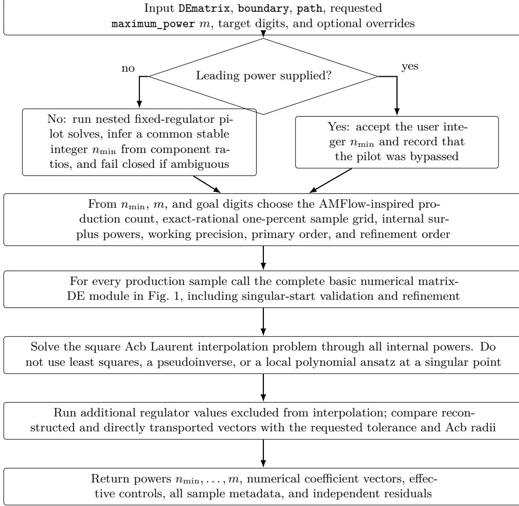
Figure 2: Semi-analytic regulator-series workflow. The basic NDE node is exactly Fig. 1 and is not expanded again. The AMFlow error estimate, automatic \epsilon scale, surplus orders, precision rules, pilot, square interpolation, and validation are detailed in Sec. 6.5; the complete optional parameter list is in Table 6 of Sec. 6.6.
