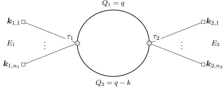
Figure 1. Feynman rules of a de Sitter bubble with general branch signs, drawn as gray vertices. The vertex energies E_1, E_2 and the conformal times \tau_1, \tau_2 are written at the vertices. The external legs end in open squares and carry the momenta k_{1,1}, \dots, k_{1,n_1} and k_{2,1}, \dots, k_{2,n_2} . The two internal lines carry the loop momenta q and q - k .
