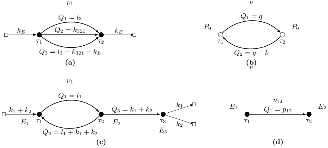
Figure 4. Example graphs. The fill colour of a vertex encodes its branch sign: black is + and white is - . (a) The two-loop sunrise of example 03: one massive full line of mass \nu_1 and two massless full lines between two + vertices; both vertices carry the same external-leg energy k_E . (b) The pure massive bubble of example 04: two massive full lines of the same mass \nu between two - vertices with vertex energy P_0 ; the loop external momentum is k . (c) The mixed bubble-plus-tree case of example 06: a massive full line of mass \nu_1 and a massless full line form the loop between v_1 and v_2 , and a massless bridge connects v_2 and v_3 ; the external legs carry k_1 + k_2 , k_1 and k_2 . (d) The two-vertex tree of example 05: a massive line of mass \nu_{12} whose momentum p_{12} is a no-loop magnitude.
