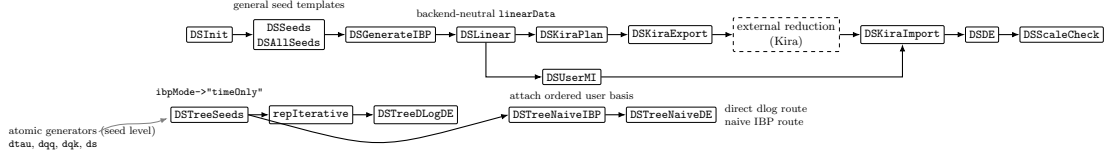
Figure 3. The public workflow of dSIBP. Full (loop) families run from DSInit through the seed, envelope and linear-system stages to the two-stage Kira export and import and to the differential-equation layer. The command DSUserMI attaches the user basis between the two reduction stages. Tree-level (timeOnly) families run through DSTreeSeeds and repIterative to DSTreeDLogDE, with the naive IBP route as an independent cross-check. The atomic generators dtau, dqq, dqk and ds are available at every stage.
