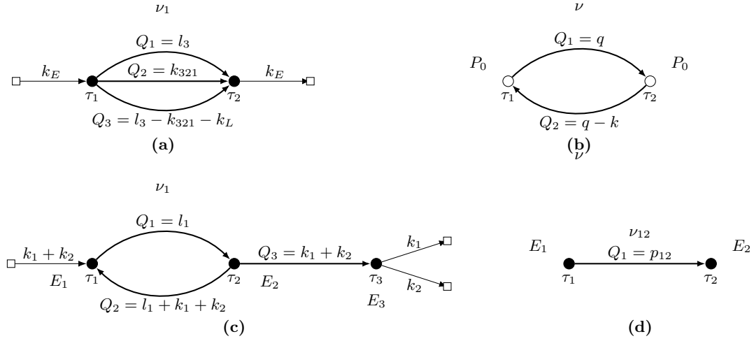
Figure 4. Example graphs. The fill colour of a vertex encodes its branch sign: black is + and white is - . (a) The two-loop sunrise of example 03: one massive full propagator of mass \nu_1 and two massless full propagators between two + vertices; both vertices carry the same external-leg energy k_E . (b) The pure massive bubble of example 04: two massive full propagators of the same mass \nu between two - vertices with vertex energy P_0 ; the loop external momentum is k . (c) The mixed bubble-plus-tree case of example 06: a massive full propagator of mass \nu_1 and a massless full propagator form the loop between v_1 and v_2 , and a massless bridge propagator connects v_2 and v_3 ; the external legs carry k_1 + k_2 , k_1 and k_2 . (d) The two-vertex tree of example 05: a massive propagator of mass \nu_{12} whose momentum p_{12} is a no-loop magnitude.
