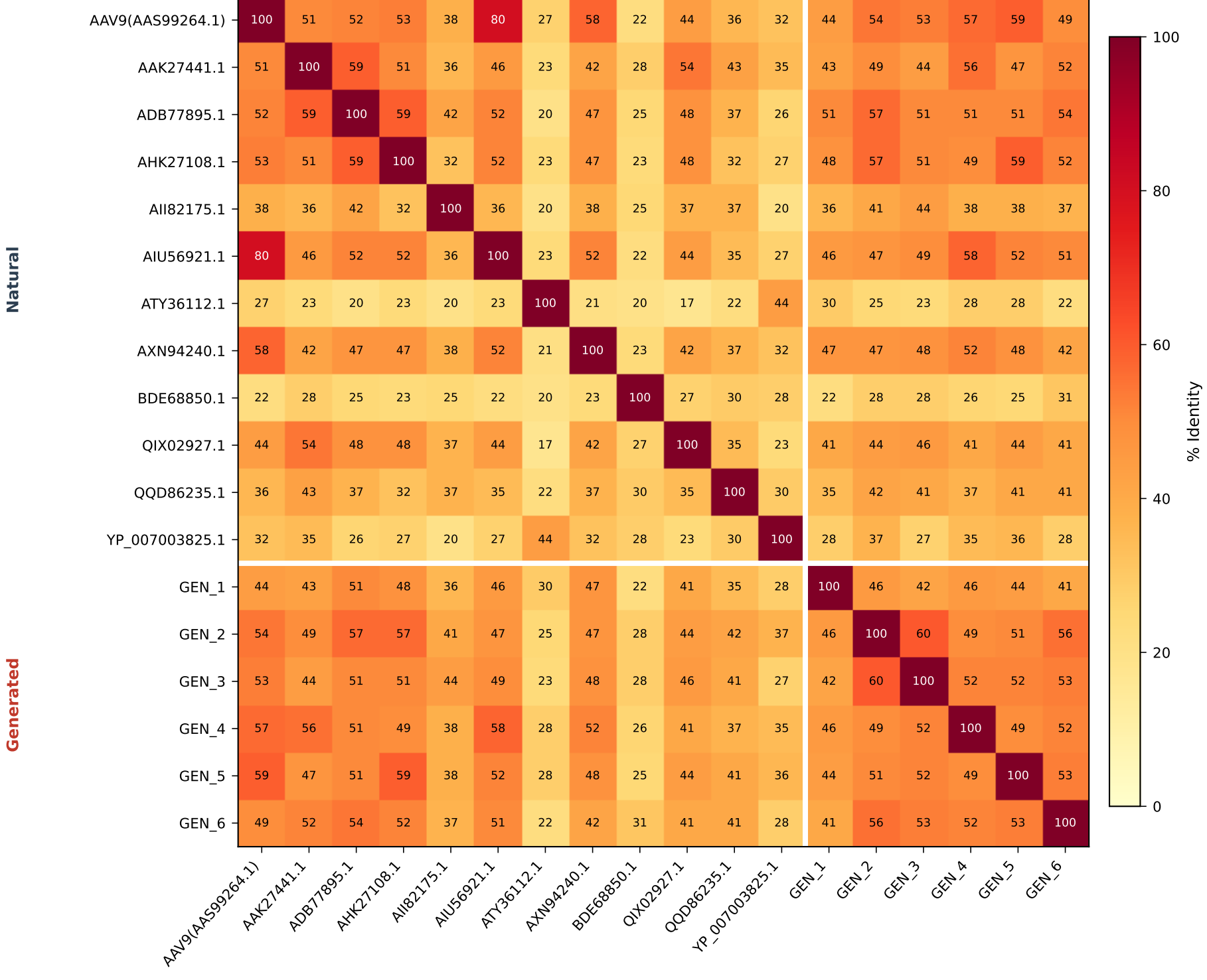
B. Sequence Identity (% identical residues)
