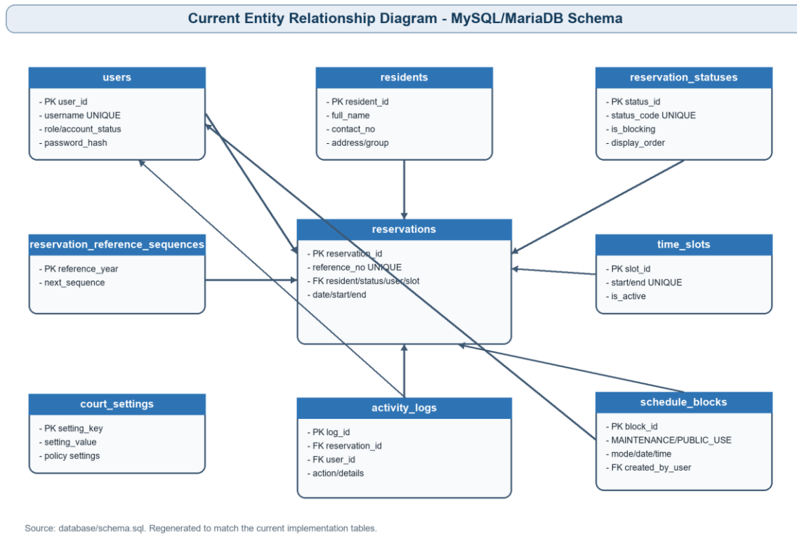
Figure 2.8. Entity Relationship Diagram of the Basketball Court Scheduling System
