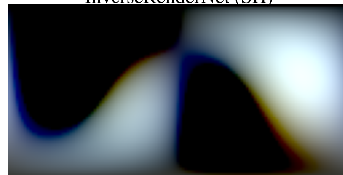
InverseRenderNet (SH)
