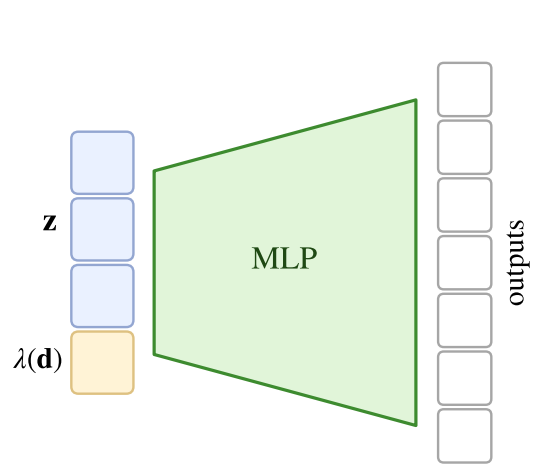
Condition-by-Concat
