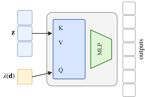
Attention
