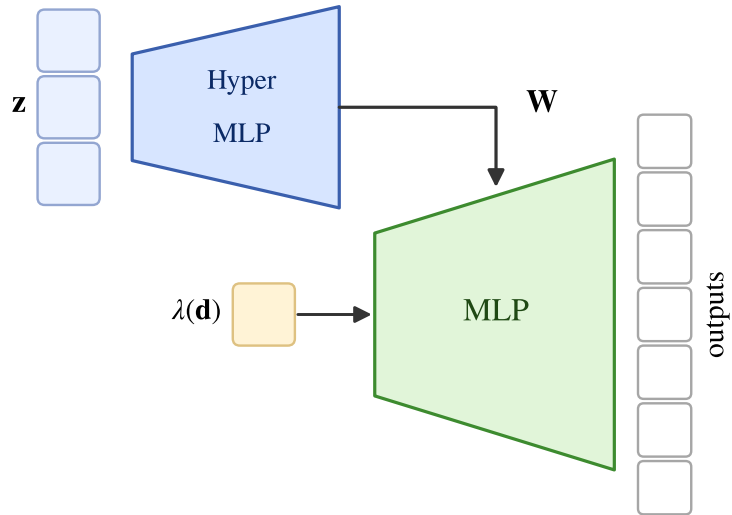
Hypernetwork
