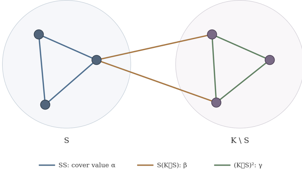
Figure 2: The three edge orbits of a pure profile.
