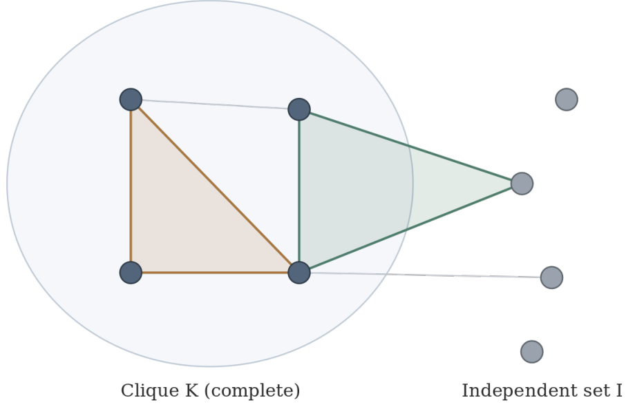
Figure 1: The two-phase fractional packing.
