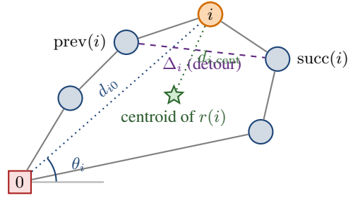
Figure 3: Geometric features attached to a node i (orange) within its current route. The detour \Delta_i measures the extra length caused by visiting i between its neighbors; (\theta_i, d_{i0}) locate i in polar coordinates around the depot; d_{i,\text{cent}} measures how far i lies from the center of gravity of its own route.
