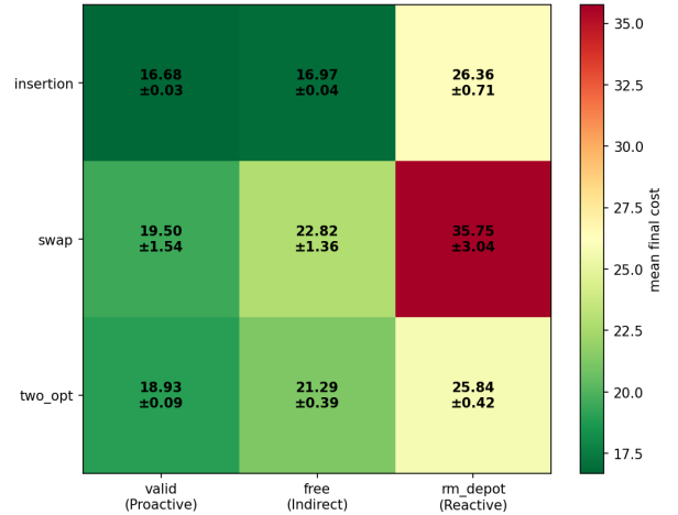
Figure 6: Mean final cost over the operator × feasibility grid (green = better). The insertion/masking corner is the optimum; the rejection column is uniformly poor across all operators.
