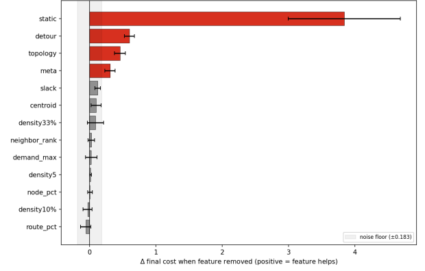
Figure 9: Leave-one-out ablation: cost increase when a single group is removed from the full set. Static dominates; detour, topology and meta are the next clearly useful groups. The shaded band is the noise floor.
