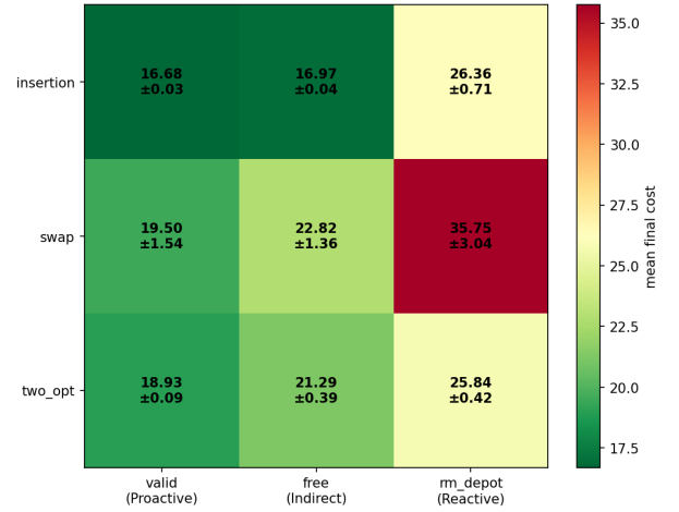
Figure 6: Mean final cost over the operator \times feasibility grid (green = better). The insertion/masking corner is the optimum; the rejection column is uniformly poor across all operators.
