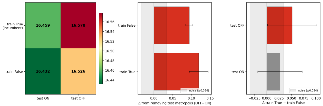
Figure 26: Metropolis train \times test cross (Table 8). Left: 2 \times 2 heatmap of mean final cost (greener = better). Center: cost of removing test-time Metropolis (off - on) at each training setting — both bars are well past the noise band, the dominant effect. Right: training-flag effect (on - off) at each deployment — the test-on bar sits inside the band (a tie), test-off just clears it.
