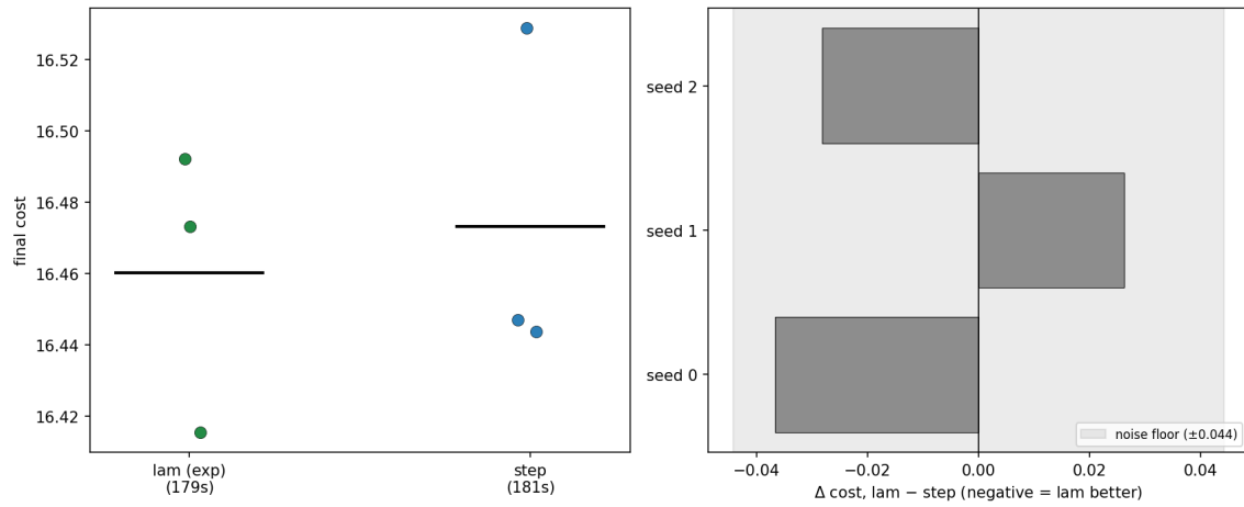
Figure 25: Cooling-schedule comparison (Table 6). Left: per-seed final cost for the two schedules (black bars = means); the clusters overlap heavily. Right: per-seed paired \Delta (geometric - step) — every bar lies inside the noise band and the sign is not consistent, the signature of a tie rather than an effect.
