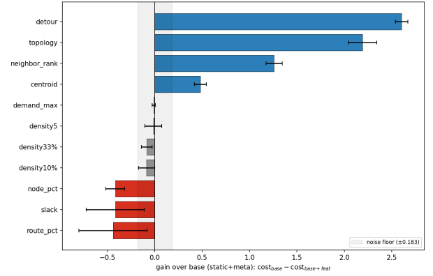
Figure 10: Isolation ablation: gain from adding a single group to the static+meta base. Detour, topology and the neighbor ranks carry most of the standalone signal; the capacity trio harms the policy when added in isolation.
