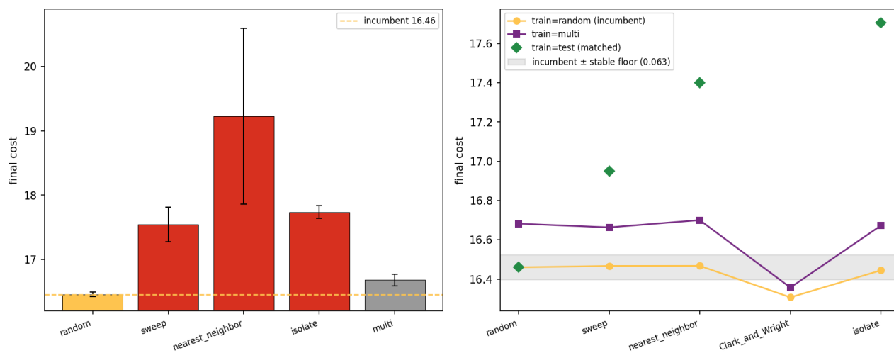
Figure 28: Left: final cost by training construction at the standard random-start deployment — random (gold) is far below the rest, with mixed (gray) a close second. Right: final cost of selected actors across the five test constructions: the random-trained actor (gold) is nearly flat and mostly inside the stable-floor band, the mixed actor (purple) sits uniformly a touch above it, and the matched train/test diagonal (green diamonds) climbs away — ruling out a train/test-matching explanation for the training-construction effect.
