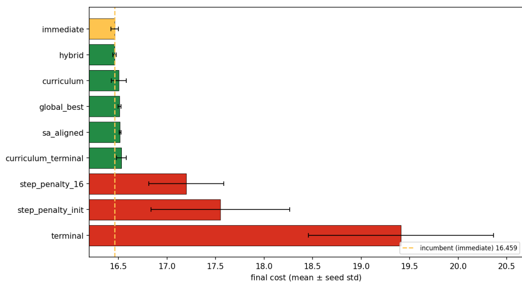
Figure 23: Full reward ranking (Table 5; mean \pm seed std, best at top). Gold = incumbent, green = the stable cluster within 0.15 of it, red = degraded. The three red bars (terminal and the two step-penalty schemes) are a different regime entirely: they fail to train a useful actor and carry runaway seed variance.
