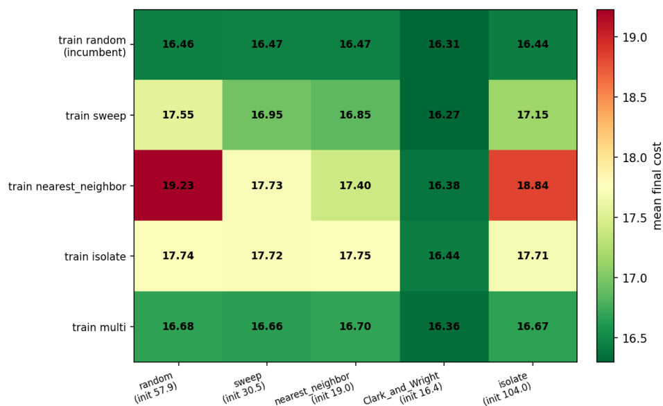
Figure 27: Initialization cross (Table 21): rows = training construction, columns = test-time construction, greener = lower final cost. The random-trained and mixed-trained rows are uniformly good; the three structured-training rows are poor and only recover in the Clarke–Wright column, where the construction itself already did the work.
