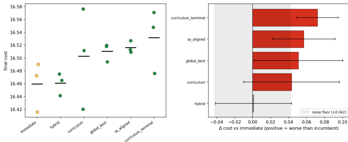
Figure 24: Zoom on the stable reward cluster. Left: per-seed final cost (black bars = means); the arms overlap heavily. Right: seed-paired \Delta against the incumbent immediate reward — the fixed mixture sits inside the noise band (a tie), the remaining dense variants are marginally but consistently above zero.
