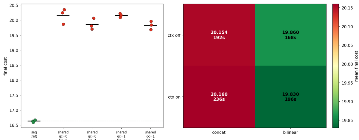
Figure 21: Shared encoder against independent scorers (Table 19). Left: per-seed final cost, incumbent reference (green) against the four shared cells (red); the dashed line marks the reference mean, and every shared seed sits far above it. Right: the shared 2 \times 2 grid — the bilinear head beats concatenation and context is roughly neutral, but all four cells are \approx 3 units worse than the reference.
