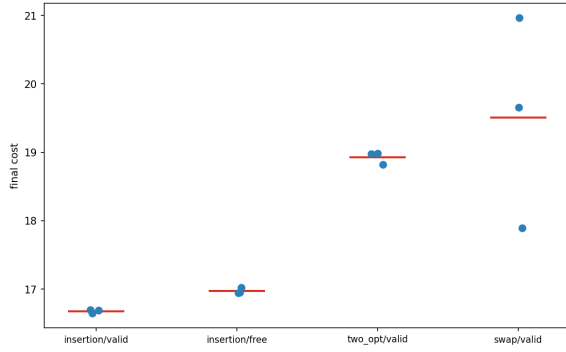
Figure 8: Per-seed final cost for the four best cells. The winning cell is tightly clustered; seed variance grows quickly as quality drops.
