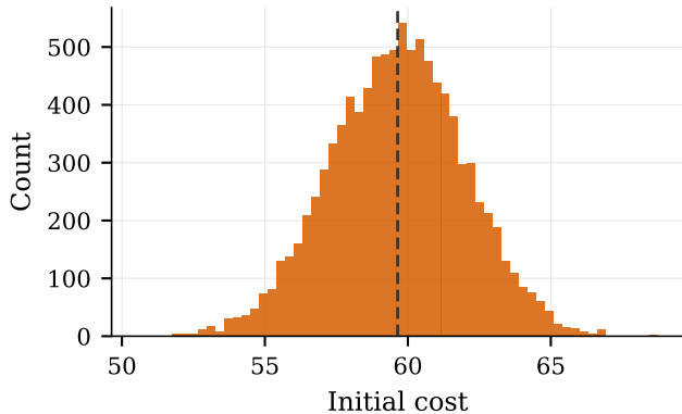
(a) random inits (mean 59.6)
