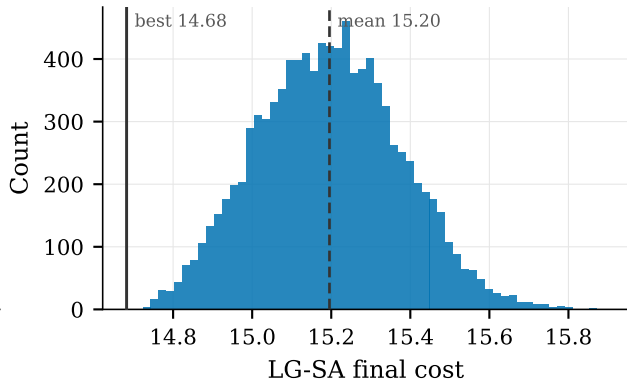
(b) after 10,000 steps
