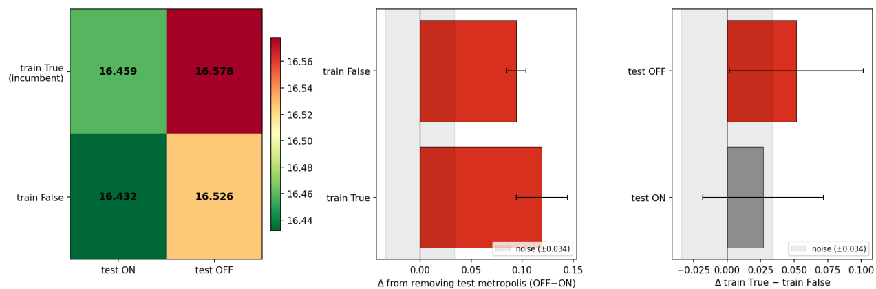
Figure 31: Metropolis train \times test cross (Table 17). Left: 2 \times 2 heatmap of mean final cost (greener = better). Center: cost of removing test-time Metropolis (off – on) at each training setting — both bars are well past the noise band, the dominant effect. Right: training-flag effect (on – off) at each deployment — the test-on bar sits inside the band (a tie), test-off just clears it.
