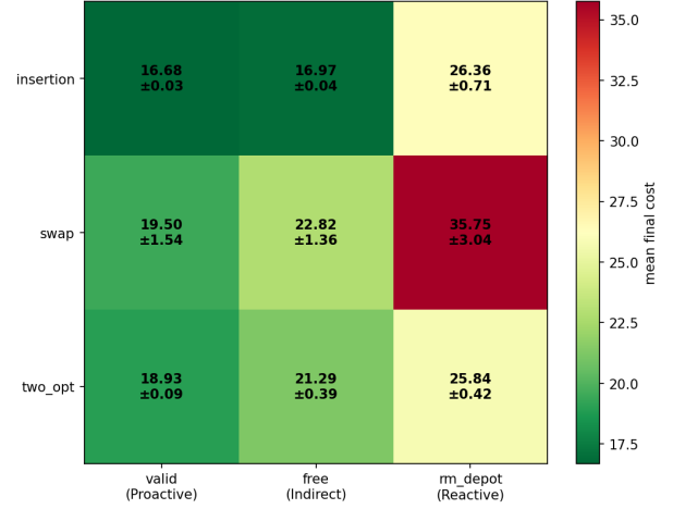
Figure 8: Mean final cost over the operator \times feasibility grid (green = better). The insertion/masking corner is the optimum; the rejection column is uniformly poor across all operators.
