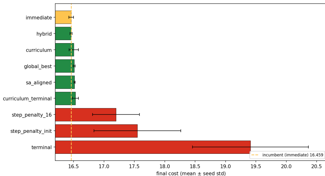
Figure 28: Full reward ranking (Table 15; mean \pm seed std, best at top). Gold = incumbent, green = the stable cluster within 0.15 of it, red = degraded. The three red bars (terminal and the two step-penalty schemes) are a different regime entirely: they fail to train a useful actor and carry runaway seed variance.
