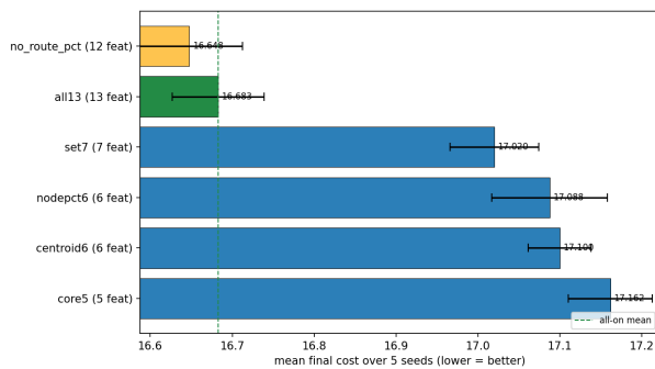
Figure 17: Best-set validation (Table 3): candidate sets ranked at 5 seeds. The 12-group set (gold) and the full set (green) tie at the top; every coarsely pruned set (blue) is clearly worse.
