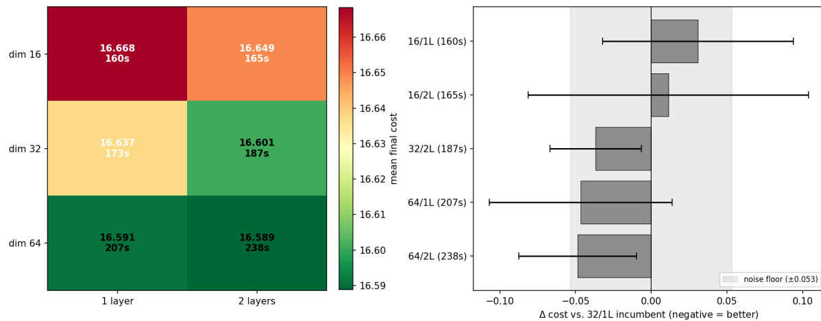
Figure 23: Actor capacity grid (Table 12). Left: mean final cost and wall-clock per cell (green = better). Right: seed-paired \Delta against the 32 \times 1 incumbent — every cell falls inside the shaded noise band, so no capacity change is a significant win.
