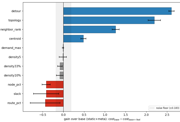
Figure 13: Isolation ablation: gain from adding a single group to the static+meta base. Detour, topology and the neighbor ranks carry most of the standalone signal; the capacity trio harms the policy when added in isolation.
