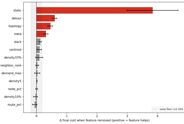
Figure 12: Leave-one-out ablation: cost increase when a single group is removed from the full set. Static dominates; detour, topology and meta are the next clearly useful groups. The shaded band is the noise floor.
