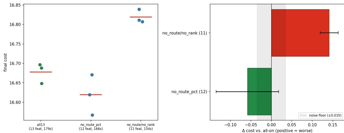
Figure 20: Targeted refinements (Table 10). Left: per-seed final cost — dropping the load ratio overlaps the full set, while additionally dropping the neighbor ranks lifts the whole cluster. Right: seed-paired \Delta vs. the full set — the load-ratio removal (green) sits inside the noise floor, the neighbor-rank removal (red) clears it decisively.
