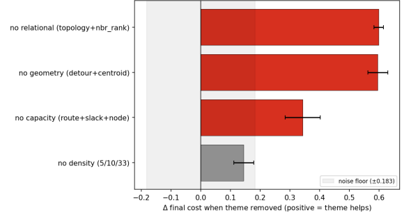
Figure 14: Thematic ablation (Table 9): removing the relational or geometry cluster costs \approx 0.6 routing units each.
