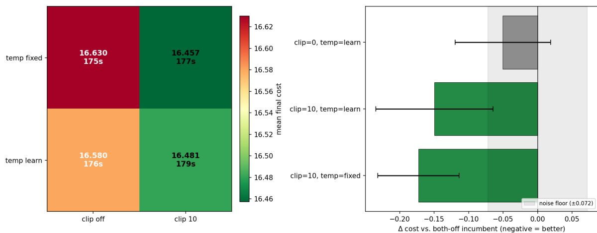
Figure 27: Distribution shaping (Table 14). Left: 2 \times 2 grid of mean final cost and time (green = better); the clipping-on, fixed-temperature cell is the best. Right: seed-paired \Delta against the both-off incumbent — only logit clipping escapes the noise band, and stacking the learnable temperature on top of it does not help.
