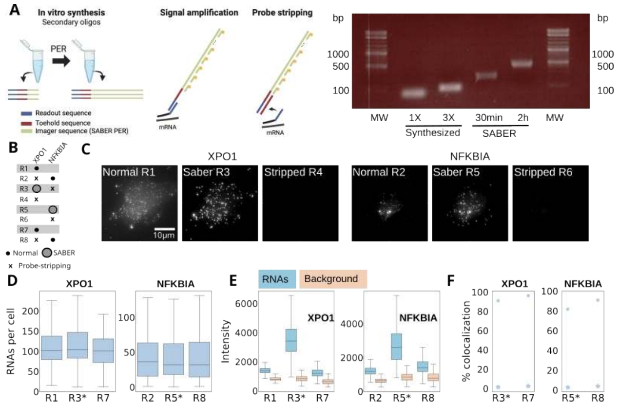
Figure 3. Signal amplification with SABER across hybridization rounds. A SABER amplifies a specific sequence by serving as a binding region for imaging oligos. Hybridization of these oligos leads to signal amplification. The oligo also contains a toehold region (red) that permits probe stripping. 2% agarose gel electrophoresis shows readout oligos with either 1 or 3 repeats, or SABER amplification with two durations (30 min and 2 h). Gel was visualized using a Fisher Bioblock Scientific UV imaging system. Full-gel image was captured on thermal paper and subsequently digitized. B Hybridization conditions for the eight rounds (R1-R8): small, filled dots indicate a standard FISH; larger dots indicate SABER FISH; x indicates stripping of the previous round. C Images of the same cell across different hybridization rounds. Images for the same gene are shown with the same intensity scaling. D RNA levels per cell across rounds. SABER runs are indicated with an asterisk. Boxplots: central line = median; box = Interquartile range (Q1–Q3); whiskers = max/min data points within 1.5× IQR. Outliers excluded. E Quantification of intensities of RNA and background across rounds. SABER runs are indicated with an asterisk. Boxplots: central line = median; box = Interquartile range (Q1–Q3); whiskers = max/min data points within 1.5× IQR. Outliers excluded. F Gene colocalization across imaging rounds. Colocalization of XPO1 and NFKB1A detections against reference detections from round 1 ( XPO1 ) and round 2 ( NFKB1A ): colocalization between the same gene is shown with a circle, between different genes with a star. These colocalization values for each condition (circle or stars) are calculated by pooling n=25 fields of view within the experiment. Small points represent colocalization coefficients for individual fields of view to indicate spatial variability. Note that the aggregated value differs in theory from the arithmetic mean of individual fields of view, as the ratio of sums is not mathematically equivalent to the mean of ratios.
