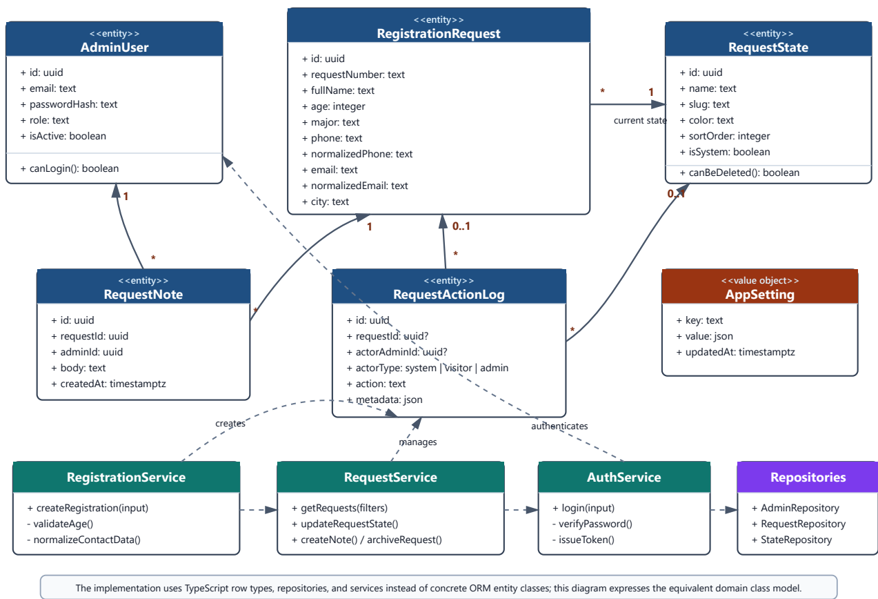
Event Registration System - Class Diagram
