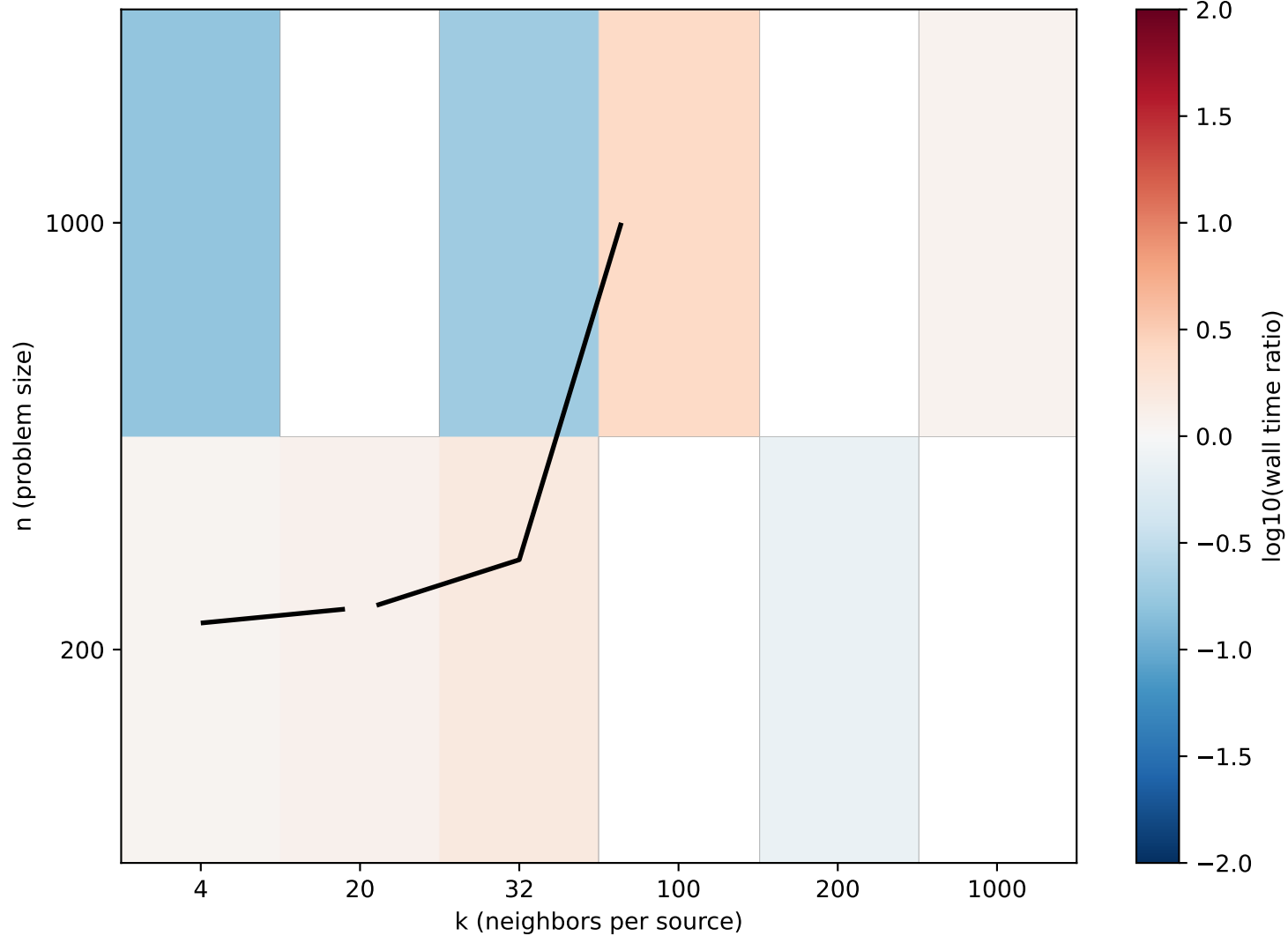
LEMON / Bonneel wall-time ratio (contour = crossover)
