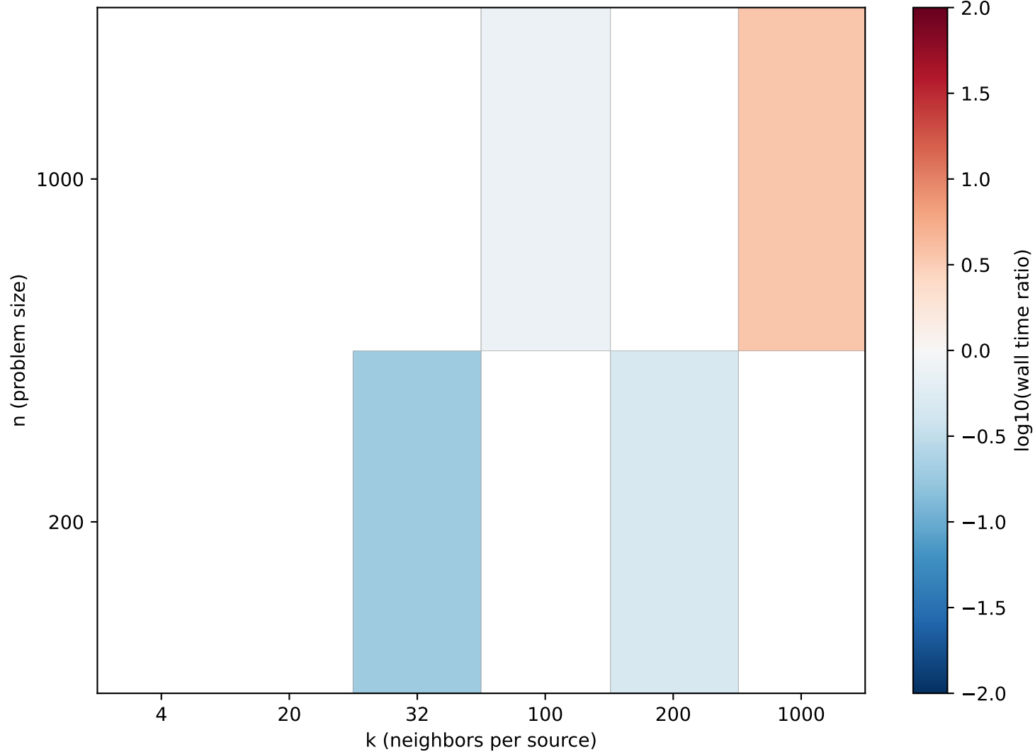
OR-Tools / LEMON wall-time ratio (contour = crossover)
