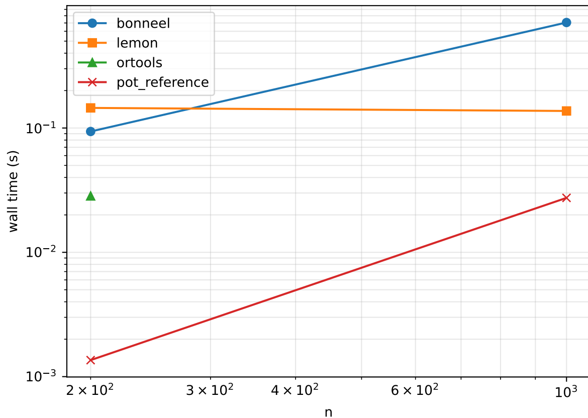
Wall time vs n at k=32
