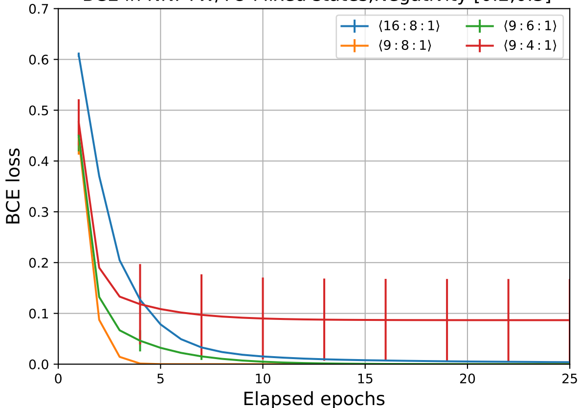
BCE in NN. TW/TO Mixed states, Negativity [0.2,0.3]
